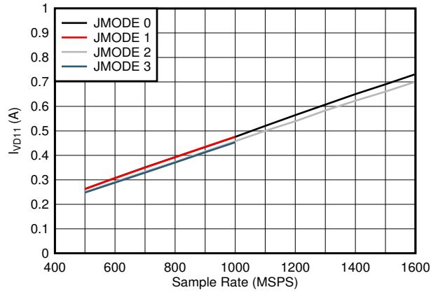
图 5-85. Quad Channel, I_{VD11} vs F_S and JMODE 0 - 3
