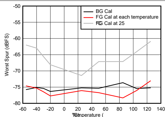
图 5-68. Worst Spur vs Temperature
