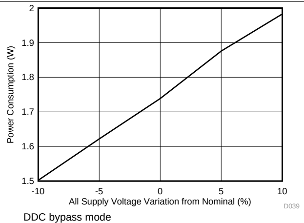
Figure 26. Power Consumption vs Supply Voltage
