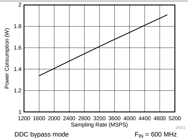
Figure 24. Power Consumption vs Sampling Rate
