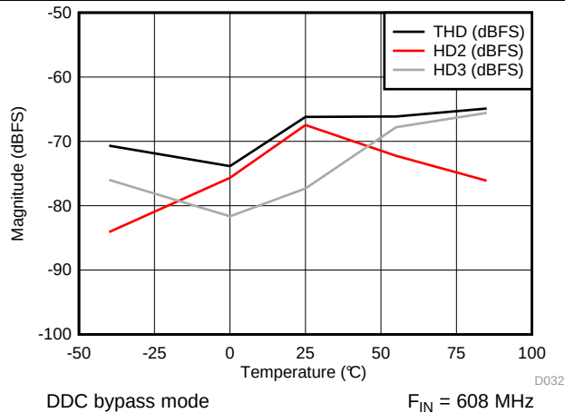
Figure 21. THD, H2, H3 vs Temperature - F_{IN} = 607.77\text{MHz}
