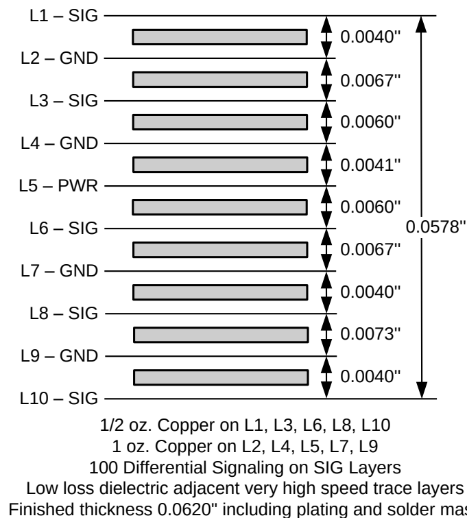
图 102. ADC12J4000 Typical Stackup — 10 Layer Board
