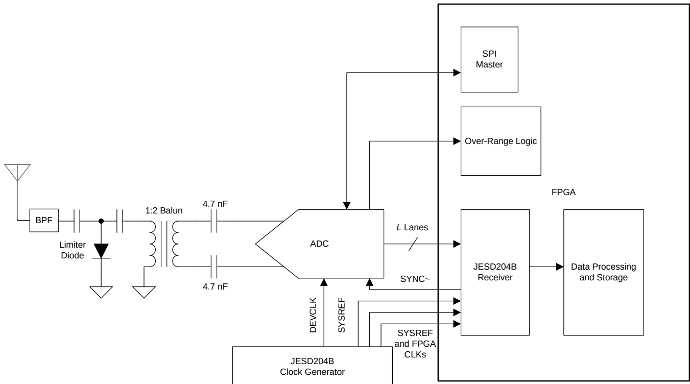
图 94. Simplified Schematic
