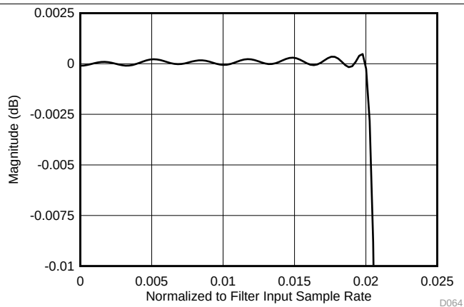
Figure 58. Decimate by 16 - Passband Response
