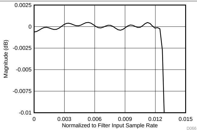
Figure 60. Decimate by 20 - Passband Response
