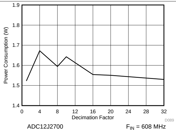
Figure 20. Power Consumption vs Decimation Setting
