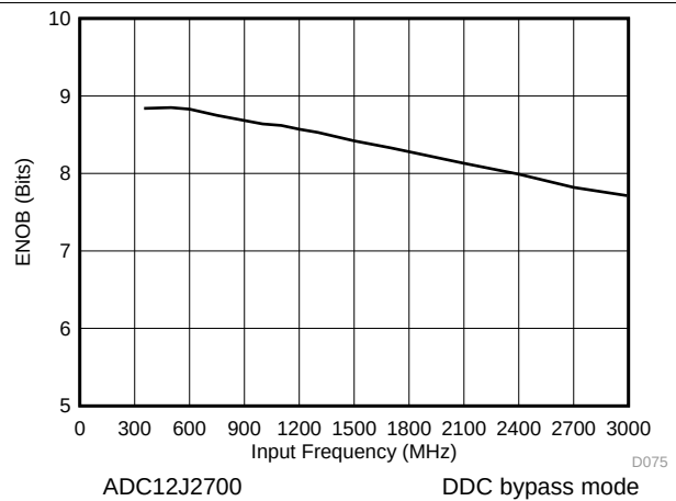
Figure 12. ENOB vs Input Frequency
