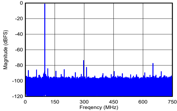
图 5-134. Single-Tone FFT at f_{IN} = 99\text{MHz} , A_{IN} = -1\text{dBFS}
