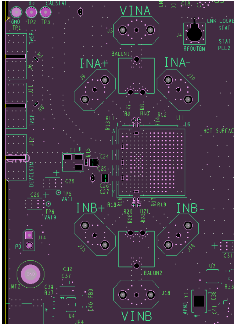
图 7-13. GND1 Cutouts to Optimize Impedance of Component Pads
