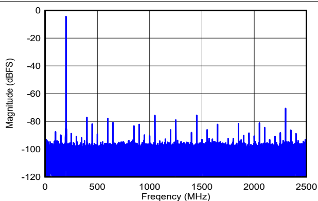
图 7-5. 200MHz, Sine-Wave Frequency Domain (FFT) for 5GSPS, Single-Channel Oscilloscope
