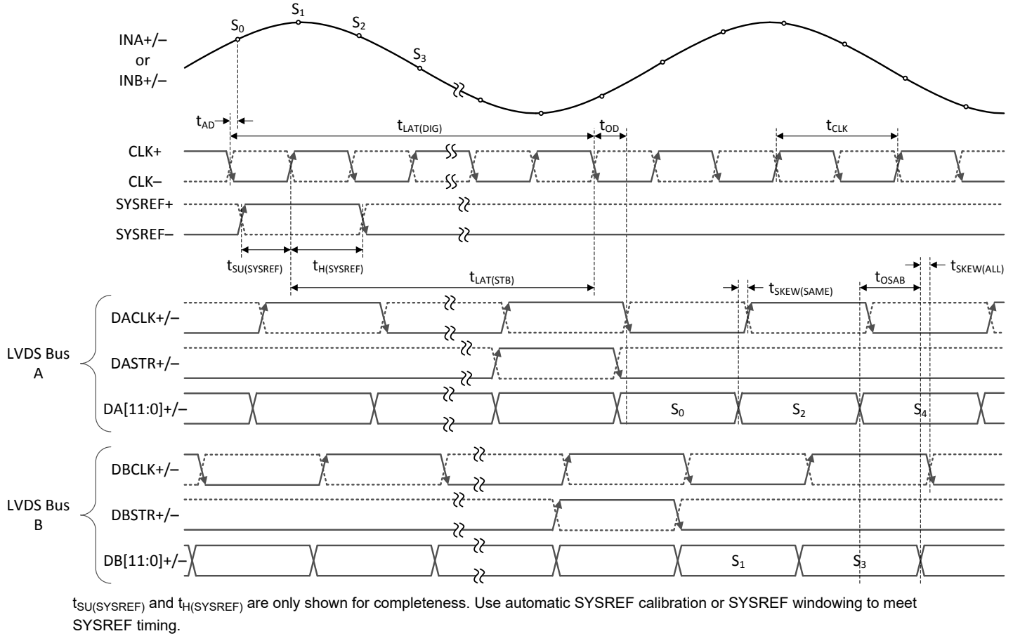
图 5-4. Single-Channel, 2-Bus, Staggered-Mode Timing (LDEMUX = 0, DES_EN = 1, LALIGNED = 0)
