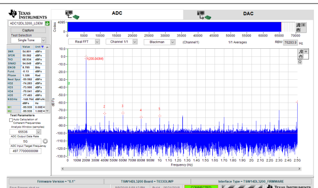
图 8-8. 200-MHz, Sine-Wave Frequency Domain (FFT) for 5-GSPS, Single-Channel Oscilloscope
