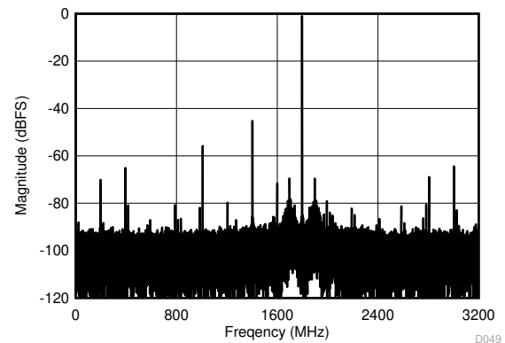
图 6-43. Single-Tone FFT at f_{IN} = 4997\text{ MHz} , A_{IN} = -1\text{ dBFS}
