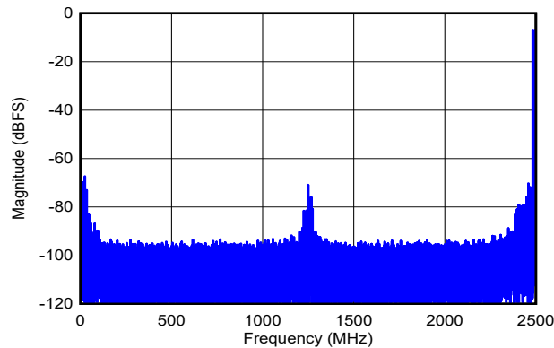
图 5-260. Two-Tone FFT at f_{IN} = 797\text{MHz} , A_{IN} = -1\text{dBFS}
