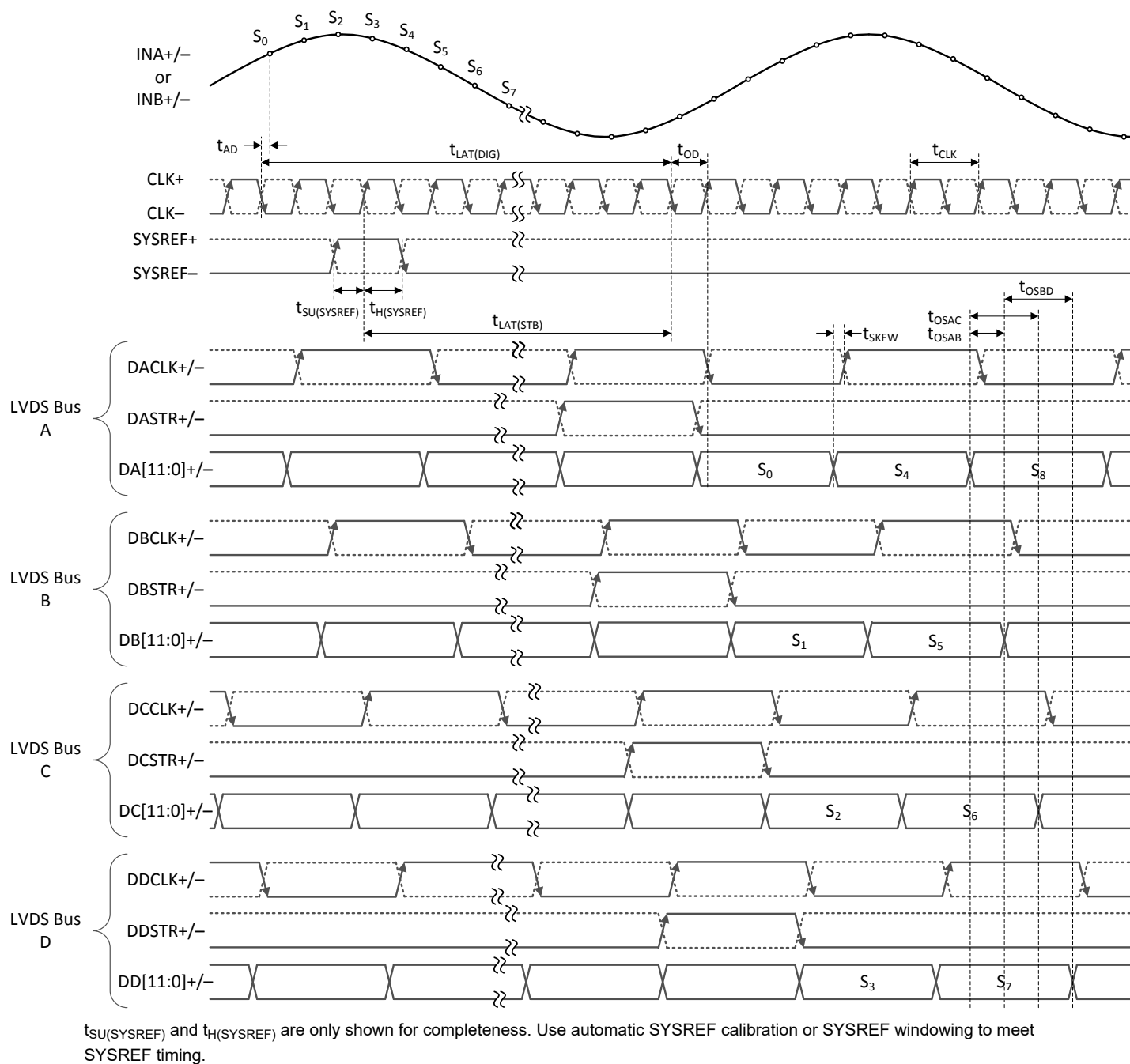
图 5-6. Single-Channel, 4-Bus, Staggered-Mode Timing (LDEMUX = 1, DES_EN = 1, LALIGNED = 0)
