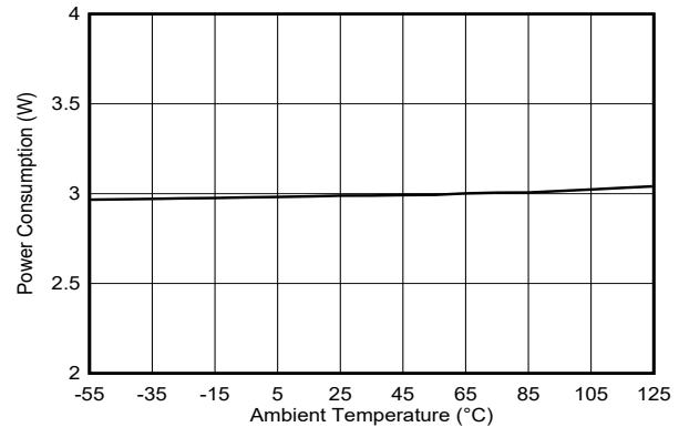
图 5-277. Power Consumption vs Temperature
