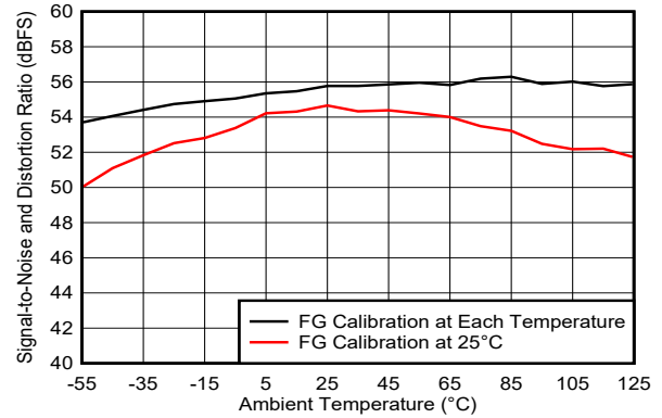
图 5-271. SINAD vs Temperature and Calibration Mode
