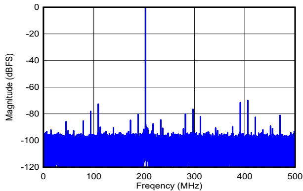
图 5-86. Single-Tone FFT at f_{\text{IN}} = 797\text{MHz} , A_{\text{IN}} = -1\text{dBFS}
