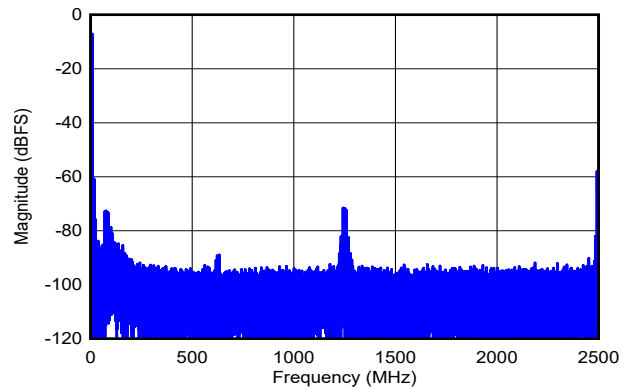
图 5-261. Two-Tone FFT at f_{IN} = 2488\text{MHz} , A_{IN} = -1\text{dBFS}
