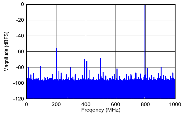
图 5-87. Single-Tone FFT at f_{\text{IN}} = 797\text{MHz} , A_{\text{IN}} = -1\text{dBFS}
