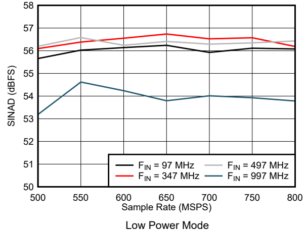
图 5-56. SINAD vs Sample Rate in Low Power Mode
