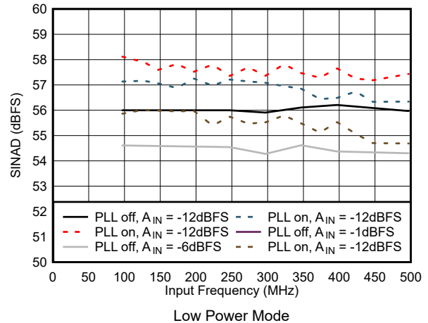
图 5-52. SINAD vs Input Frequency in Low Power Mode
