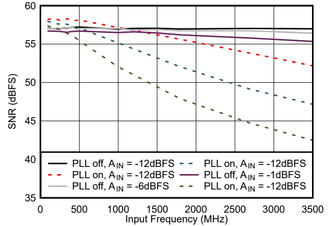
图 5-22. SNR vs Input Frequency
