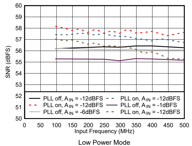
图 5-48. SNR vs Input Frequency in Low Power Mode
