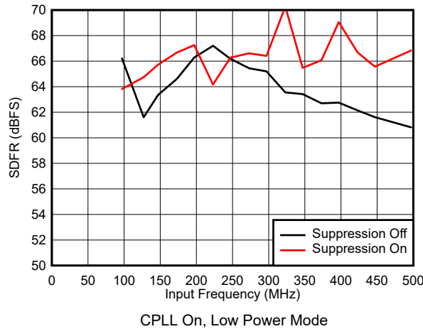
图 5-61. SFDR vs Input Frequency
