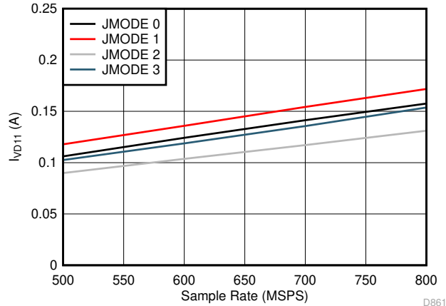
图 5-107. Single Channel, I_{VD11} vs F_S for JMODES 0 - 3
