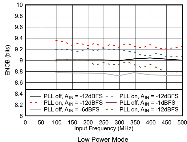
图 5-53. ENOB vs Input Frequency in Low Power Mode
