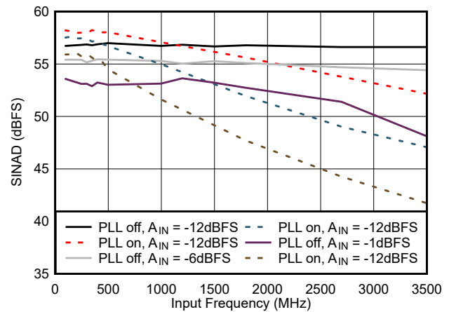
图 5-26. SINAD vs Input Frequency
