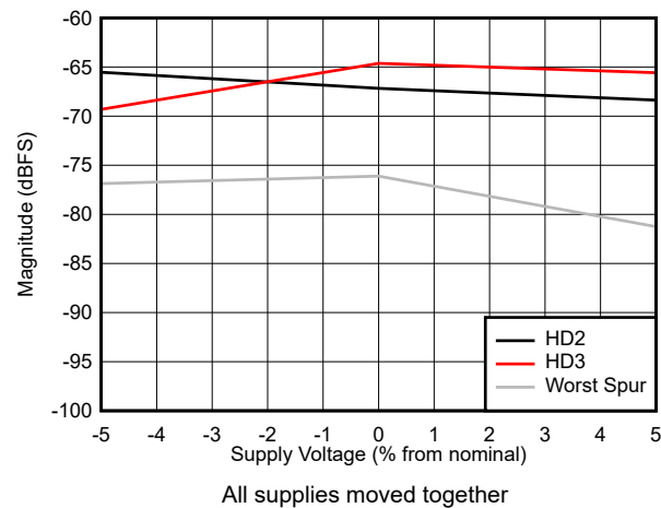
图 5-39. HD2, HD3 and worst non-HD vs Supply Voltage
