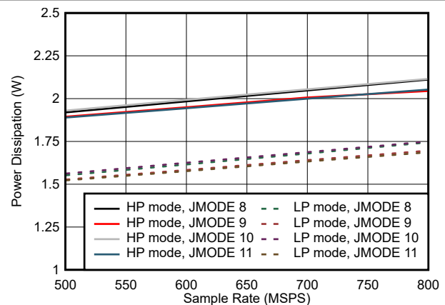
图 5-76. Quad Channel, Power Dissipation vs F_S for JMODES 8 - 11
