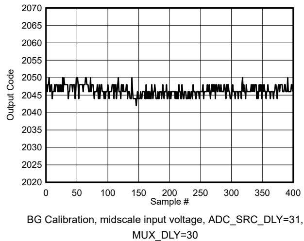
图 5-115. Background Calibration Core Transition (midscale)
