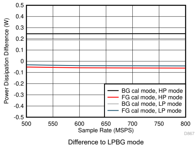
图 5-111. Single Channel, Power Dissipation vs F_S over Modes
