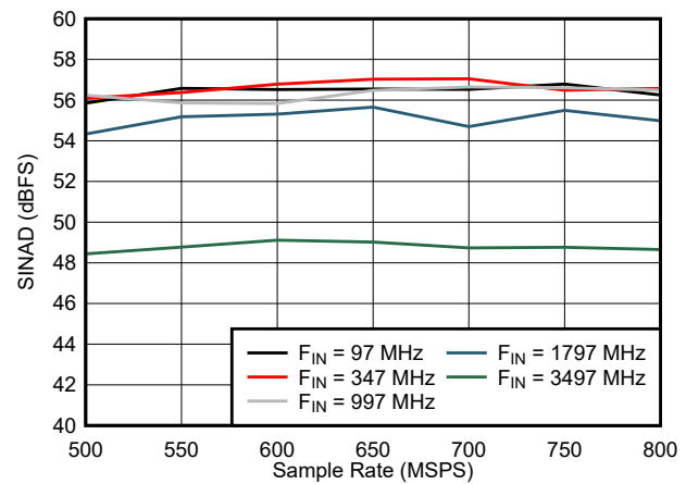
图 5-30. SINAD vs Sample Rate
