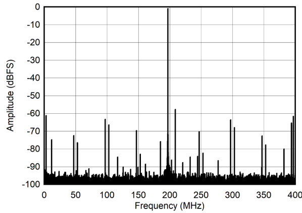
图 5-21. Single Tone FFT at 997 MHz and -1dBFS
