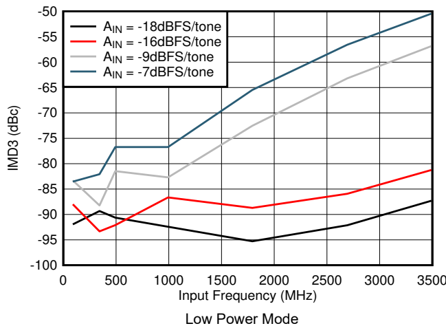
图 5-73. IMD3 vs Input Frequency in Low Power Mode
