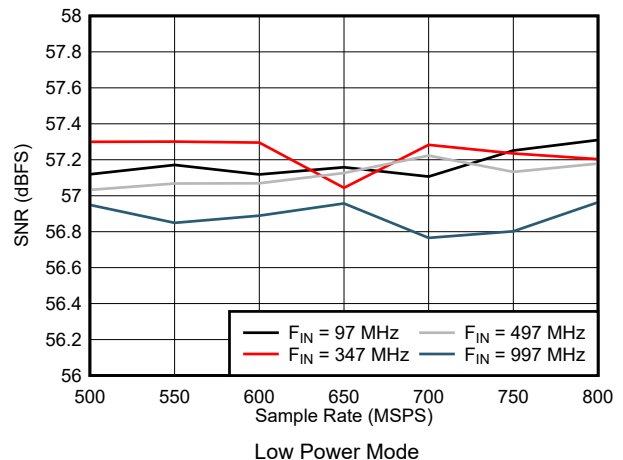
图 5-54. SNR vs Sample Rate in Low Power Mode
