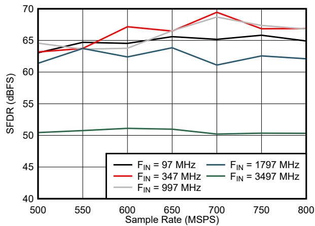
图 5-29. SFDR vs Sample Rate
