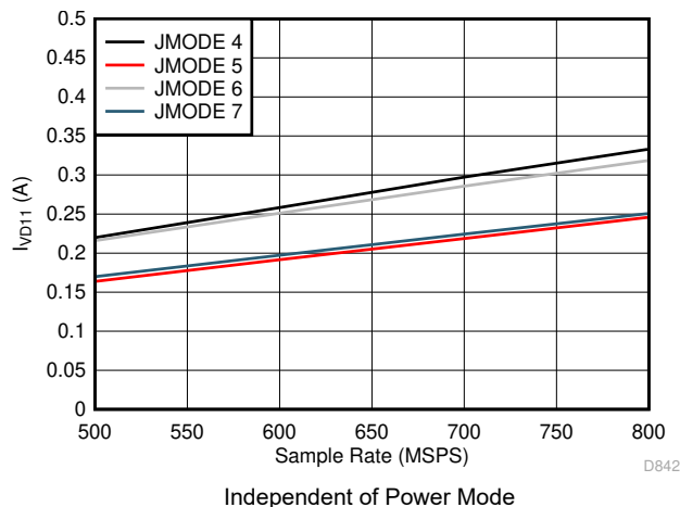
图 5-81. Quad Channel, I_{VD11} vs F_S for JMODES 4 - 7
