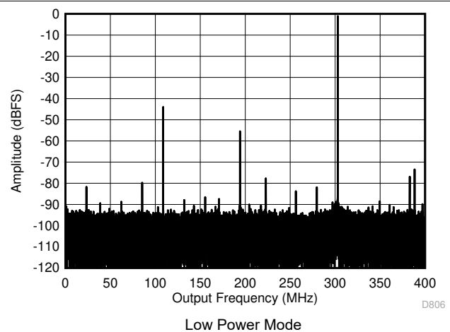
图 5-12. Single Tone FFT at 2097 MHz and -1dBFS
