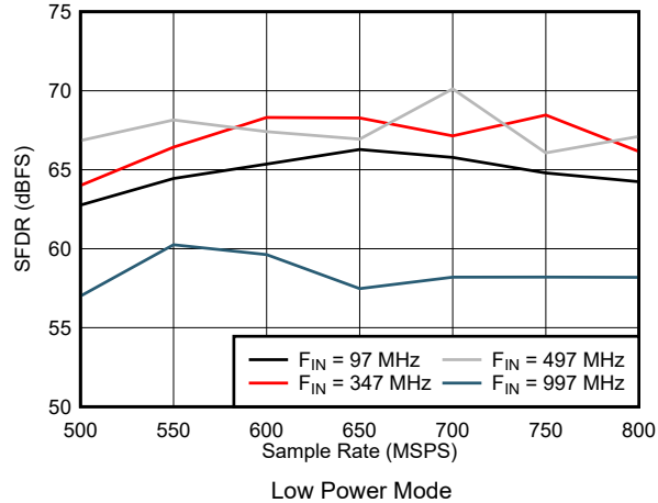
图 5-55. SFDR vs Sample Rate in Low Power Mode
