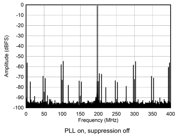
图 5-16. Single Tone FFT at 997 MHz and -1dBFS
