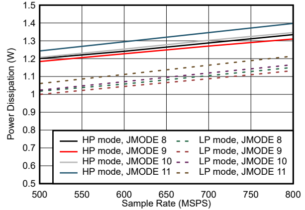
图 5-90. Dual Channel, Power Dissipation vs F_S for JMODES 8 - 11
