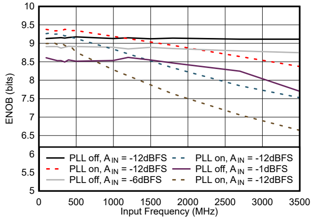
图 5-27. ENOB vs Input Frequency
