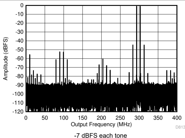
图 5-68. Two Tone FFT at 3498 MHz
