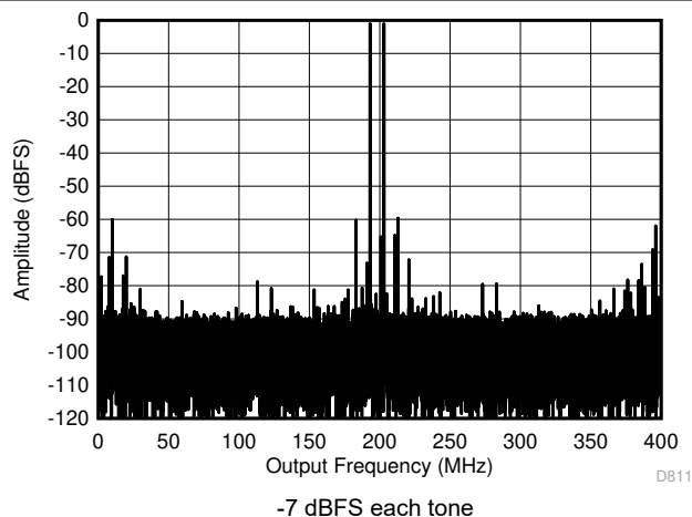
图 5-67. Two Tone FFT at 1798 MHz
