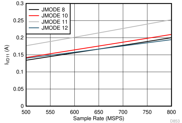
图 5-96. Dual Channel, I_{VD11} vs F_S for JMODES 8 - 12
