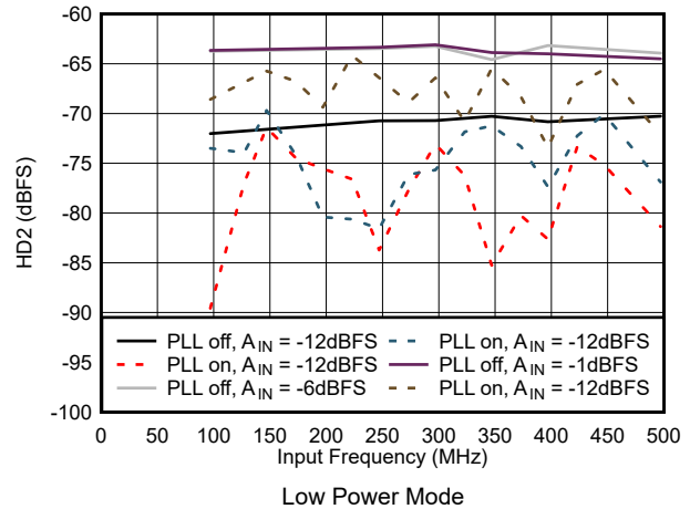
图 5-50. HD2 vs Input Frequency in Low Power Mode
