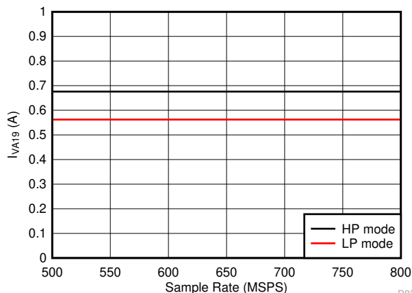
图 5-78. Quad Channel, I_{VA19} vs F_S
