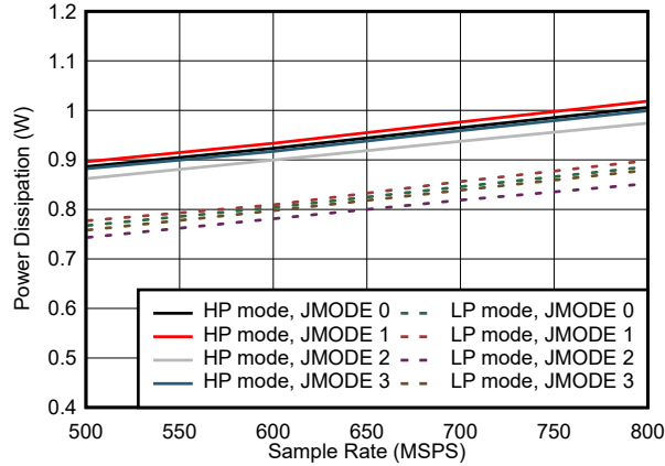
图 5-101. Dual Channel, Power Dissipation vs F_S for JMODES 0 - 3
