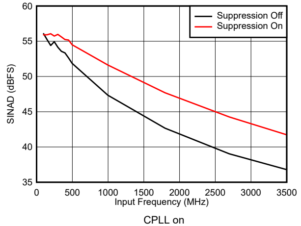
图 5-36. SINAD vs Input Frequency and Suppression
