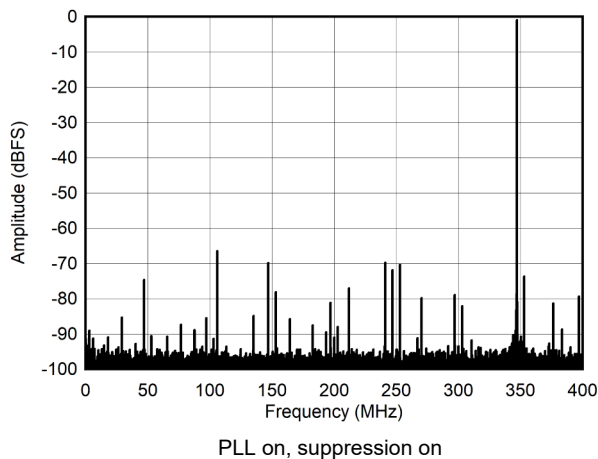
图 5-15. Single Tone FFT at 347 MHz and -1dBFS
