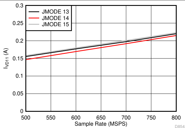
图 5-97. Dual Channel, I_{VD11} vs F_S for JMODES 13 - 15
