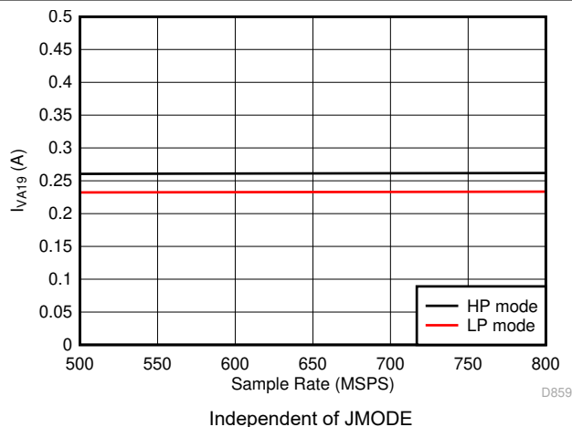
图 5-105. Single Channel, I_{VA19} vs F_S
