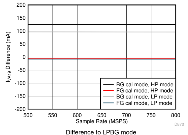
图 5-112. Single Channel, I_{VA19} vs F_S over Modes
