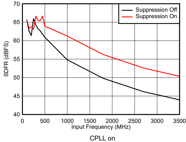
图 5-35. SFDR vs Input Frequency and Suppression
