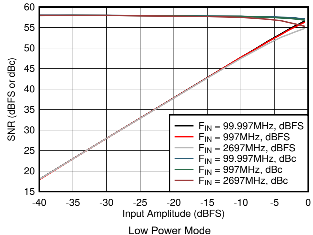
图 5-58. SNR vs Input Amplitude in Low Power Mode
