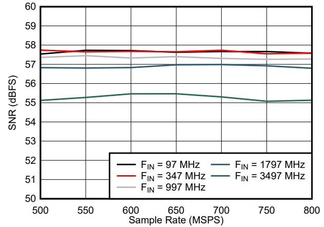
图 5-28. SNR vs Sample Rate
