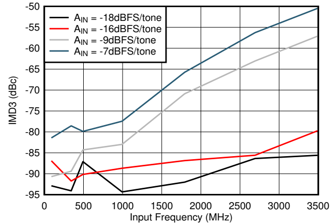
图 5-72. IMD3 vs Input Frequency
