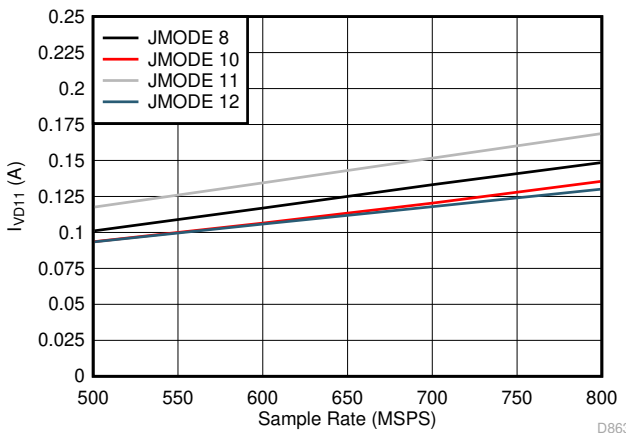
图 5-109. Single Channel, I_{VD11} vs F_S for JMODES 8 - 12
