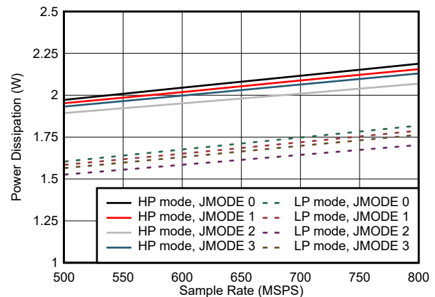
图 5-74. Quad Channel, Power Dissipation vs F_S for JMODES 0 - 3
