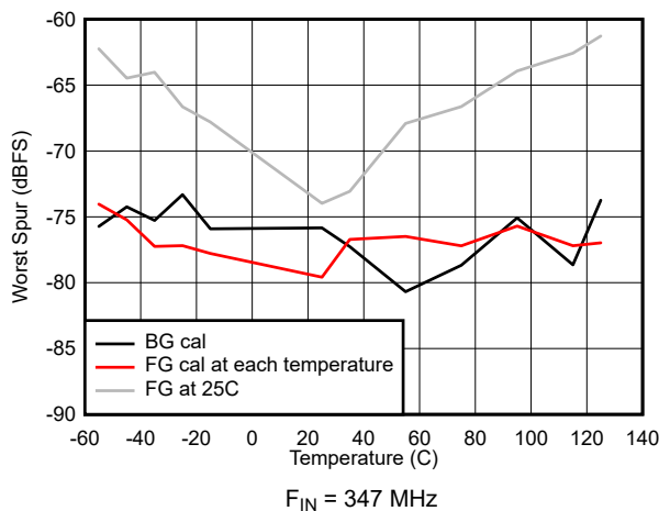
图 5-47. worst non-HD spur vs Temperature
