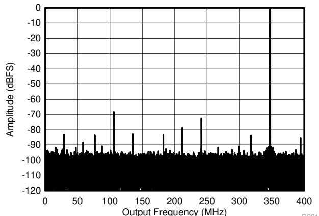
图 5-6. Single Tone FFT at 347 MHz and -1dBFS
