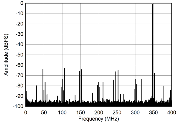
图 5-18. Single Tone FFT at 347 MHz and -1dBFS
