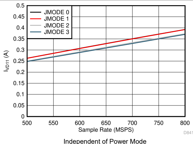
图 5-80. Quad Channel, I_{VD11} vs F_S for JMODES 0 - 3
