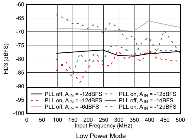
图 5-51. HD3 vs Input Frequency in Low Power Mode
