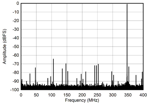
图 5-19. Single Tone FFT at 347 MHz and -1dBFS
