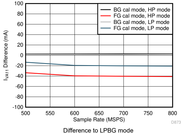
图 5-113. Single Channel, I_{VA11} vs F_S over Modes
