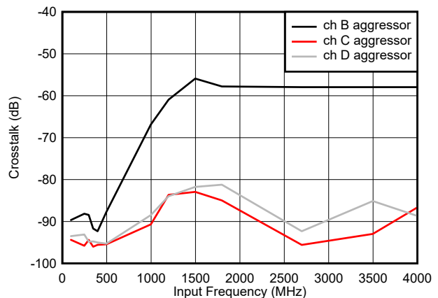
图 5-4. Crosstalk vs Input Frequency, Channel A victim
