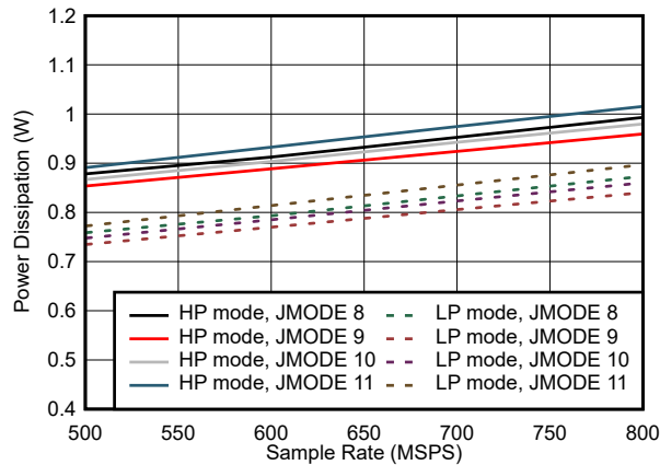
图 5-103. Single Channel, Power Dissipation vs F_S for JMODES 8 - 11
