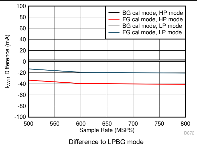
图 5-100. Dual Channel, I_{VA11} vs F_S over Modes
