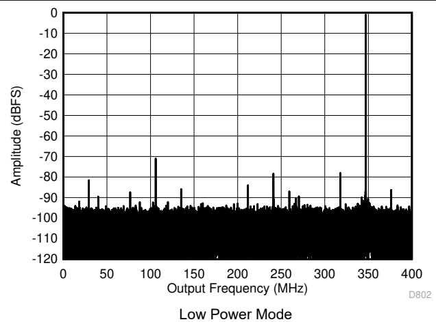
图 5-10. Single Tone FFT at 347 MHz and -1dBFS
