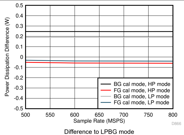
图 5-98. Dual Channel, Power Dissipation vs F_S over Modes
