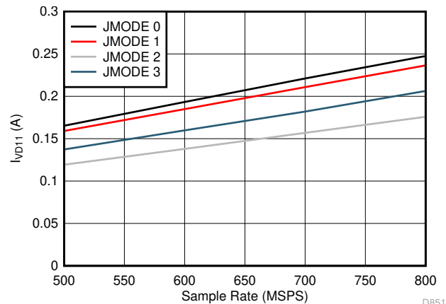
图 5-94. Dual Channel, I_{VD11} vs F_S for JMODES 0 - 3
