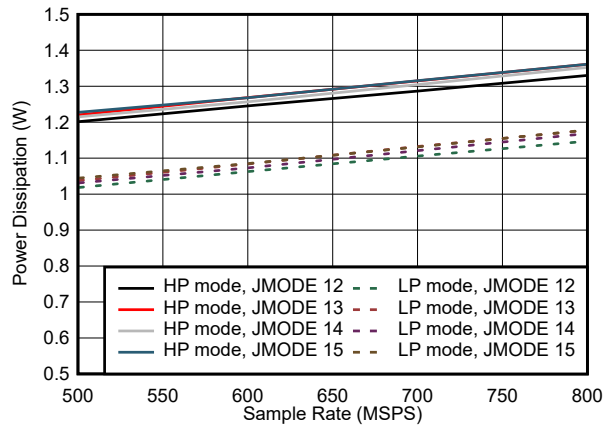
图 5-91. Dual Channel, Power Dissipation vs F_S for JMODES 12 - 15
