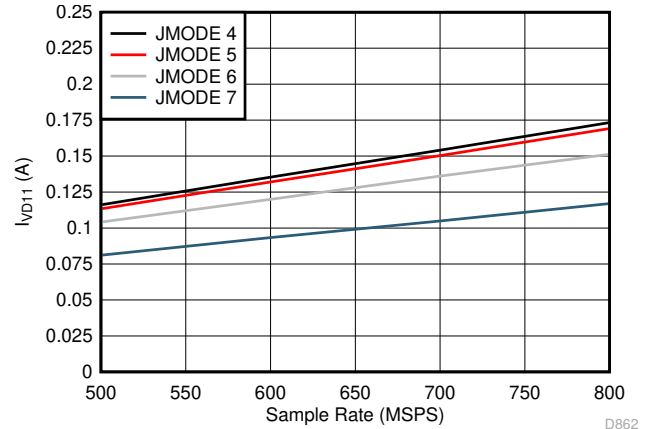
图 5-108. Single Channel, I_{VD11} vs F_S for JMODES 4 - 7
