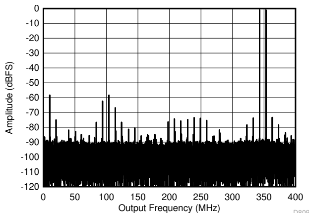
图 5-66. Two Tone FFT at 347 MHz
