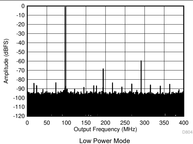
图 5-11. Single Tone FFT at 897 MHz and -1dBFS
