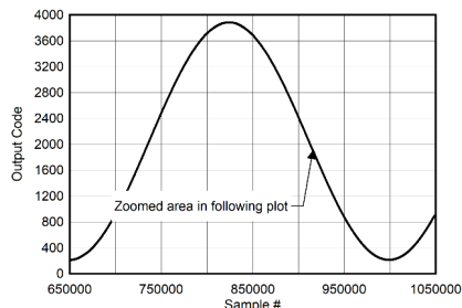
图 5-117. Background Calibration Core Transition (AC signal)
