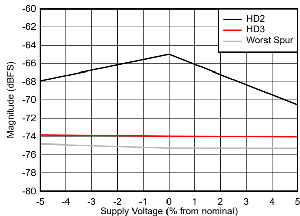
图 5-65. HD2, HD3 and worst non-HD vs Supply Voltage
