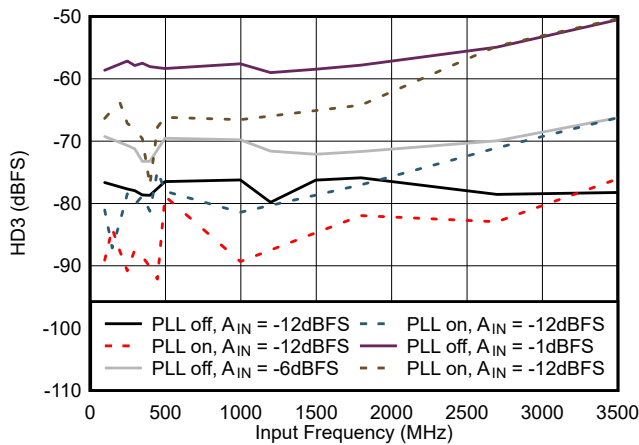
图 5-25. HD3 vs Input Frequency
