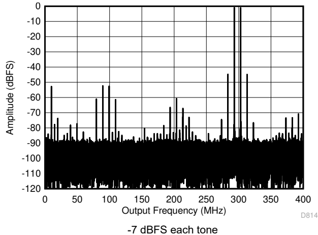
图 5-71. Two Tone FFT at 3498 MHz in Low Power Mode
