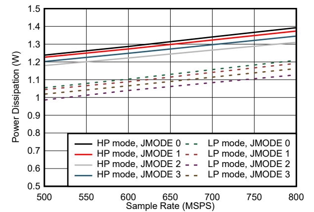
图 5-88. Dual Channel, Power Dissipation vs F_S for JMODES 0 - 3
