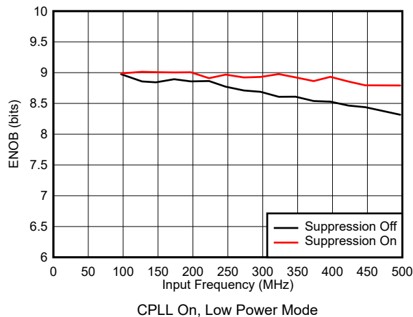
图 5-63. ENOB vs Input Frequency
