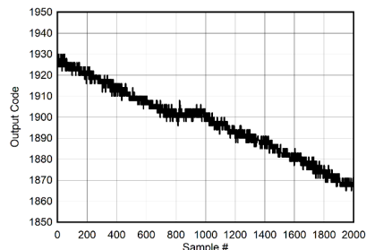
图 5-118. Background Calibration Core Transition (AC signal zoomed)
