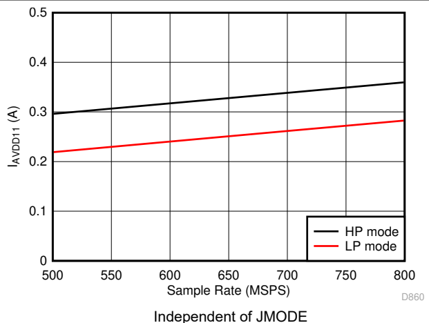
图 5-106. Single Channel, I_{VA11} vs F_S
