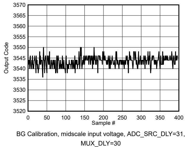
图 5-116. Background Calibration Core Transition (voltage offset)
