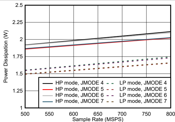
图 5-75. Quad Channel, Power Dissipation vs F_S for JMODES 4 - 7
