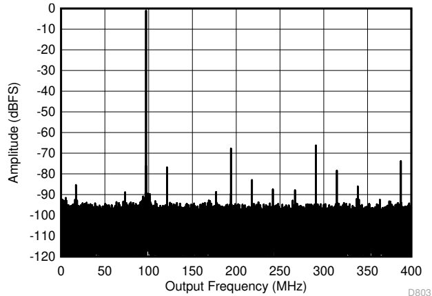
图 5-7. Single Tone FFT at 897 MHz and -1dBFS
