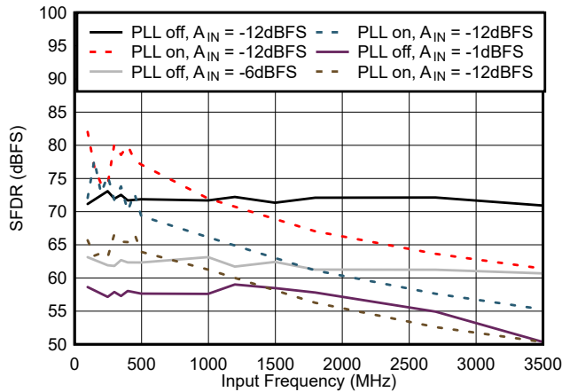
图 5-23. SFDR vs Input Frequency
