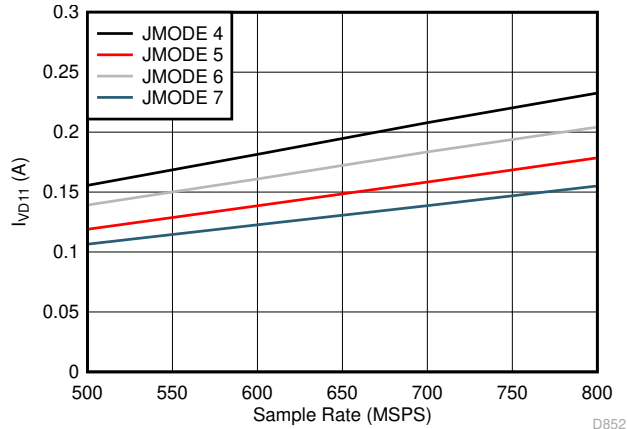
图 5-95. Dual Channel, I_{VD11} vs F_S for JMODES 4 - 7
