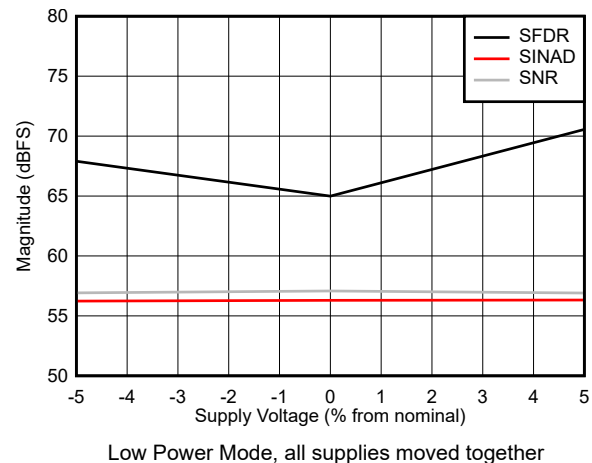
图 5-64. SNR, SFDR and SINAD vs Supply Voltage
