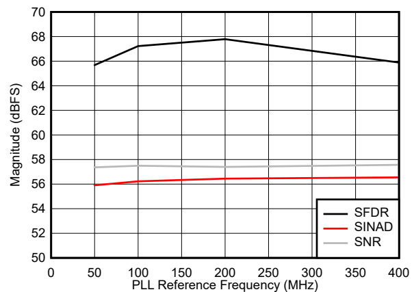
图 5-42. SNR, SFDR and SINAD vs Reference Frequency with PLL on
