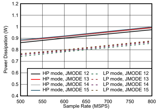
图 5-104. Single Channel, Power Dissipation vs F_S for JMODES 12 - 15
