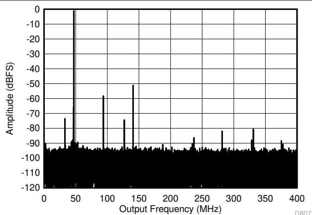
图 5-9. Single Tone FFT at 3247 MHz and -1dBFS
