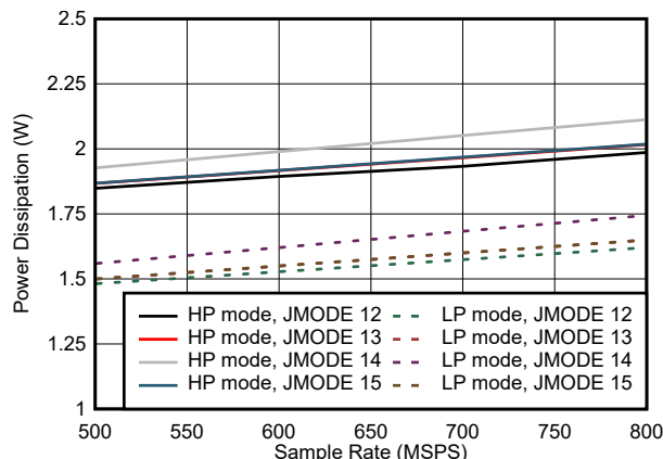
图 5-77. Quad Channel, Power Dissipation vs F_S for JMODES 12 - 15
