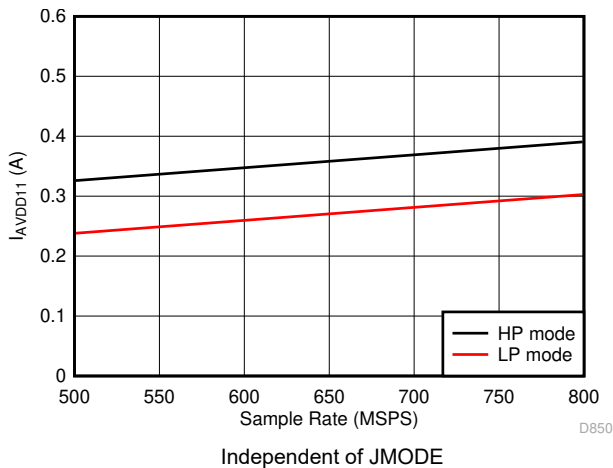
图 5-93. Dual Channel, I_{VA11} vs F_S
