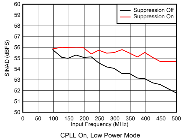
图 5-62. SINAD vs Input Frequency
