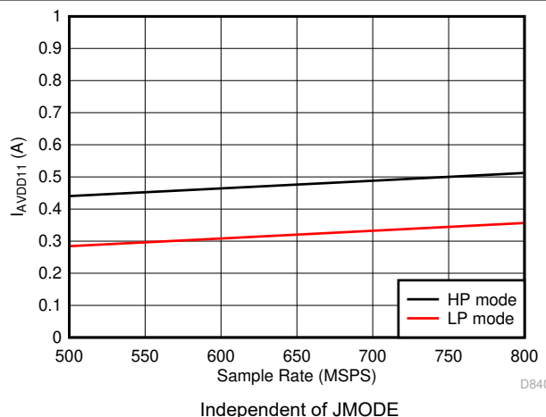
图 5-79. Quad Channel, I_{VA11} vs F_S
