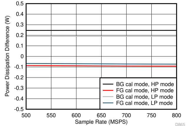
图 5-84. Quad Channel, Power Dissipation vs F_S over Modes
