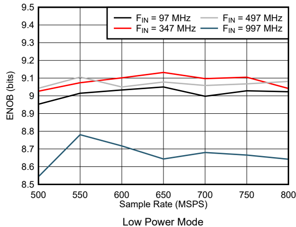
图 5-57. ENOB vs Sample Rate in Low Power Mode
