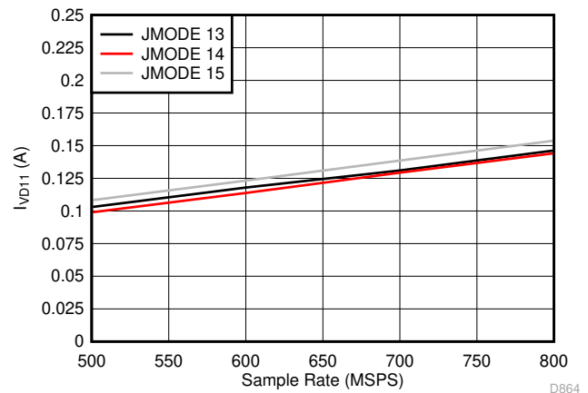
图 5-110. Single Channel, I_{VD11} vs F_S for JMODES 13 - 15
