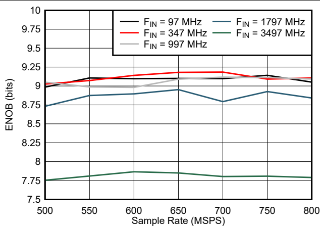
图 5-31. ENOB vs Sample Rate
