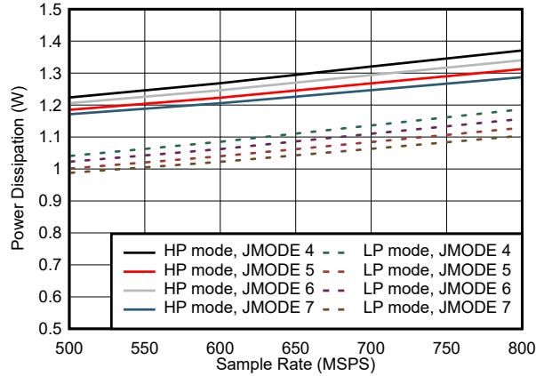
图 5-89. Dual Channel, Power Dissipation vs F_S for JMODES 4 - 7
