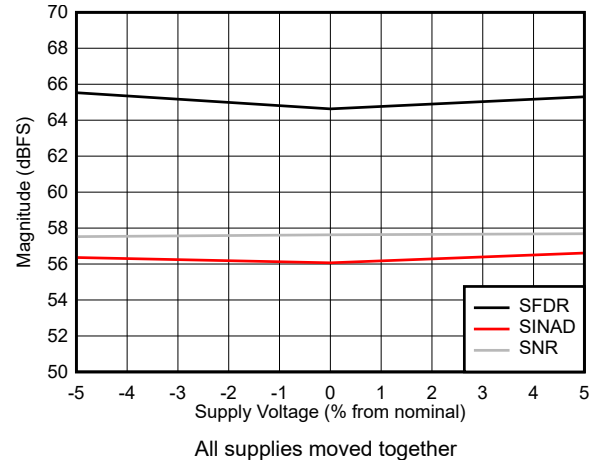
图 5-38. SNR, SFDR and SINAD vs Supply Voltage
