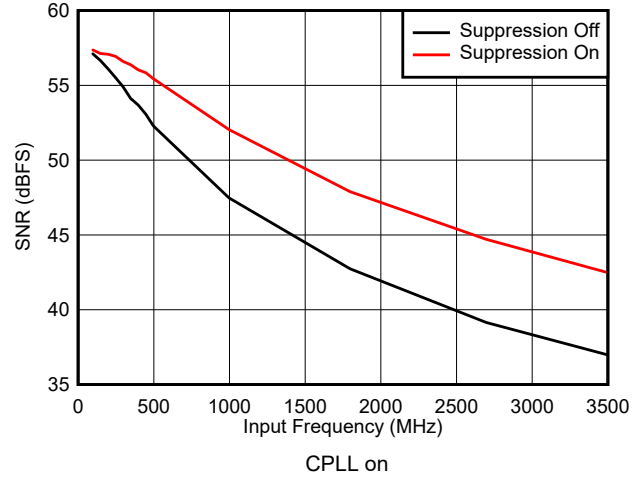
图 5-34. SNR vs Input Frequency and Suppression
