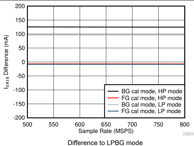
图 5-99. Dual Channel, I_{VA19} vs F_S over Modes
