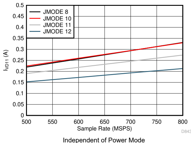
图 5-82. Quad Channel, I_{VD11} vs F_S for JMODES 8-12
