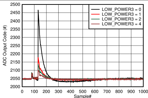
图 6-12. Background Calibration Core Transition in Low Power Mode
