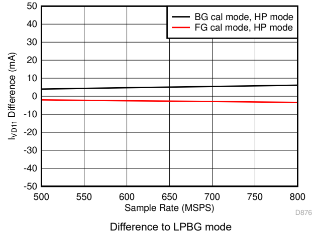
图 5-114. Single Channel, I_{VD11} vs F_S over Modes
