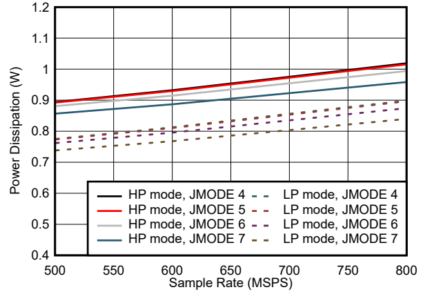
图 5-102. Single Channel, Power Dissipation vs F_S for JMODES 4 - 7
