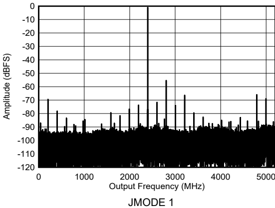
图 5-27. DES Mode: Single Tone Output Spectrum at 2397 MHz
