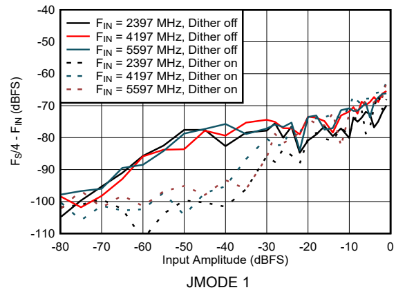
图 5-20. DES Mode: F_S/4 - F_{\text{IN}} vs Input Amplitude
