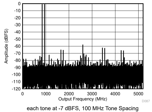
图 5-12. DES Mode: Two Tone FFT at 897 MHz
