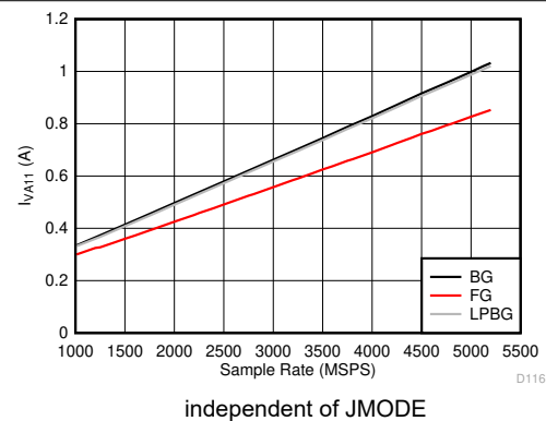
图 5-132. Dual Channel Mode: I_{VA11} vs Sample Rate
