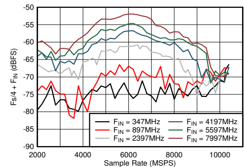
图 5-42. DES Mode: \text{Fs}/4 + F_{\text{IN}} vs Sample Rate and Input Frequency
