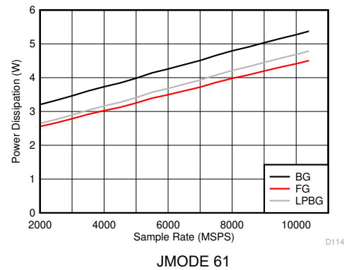
图 5-130. DES Mode: Power Dissipation vs Sample Rate
