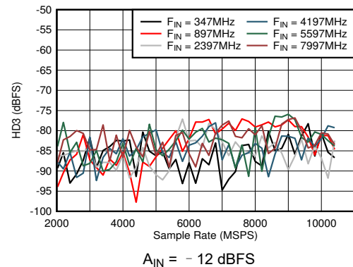
图 5-40. DES Mode: HD3 vs Sample Rate and Input Frequency
