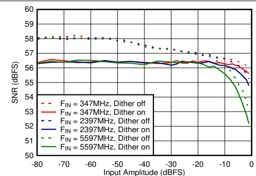
图 5-72. Dual Channel Mode: SNR vs Input Amplitude and Dither
