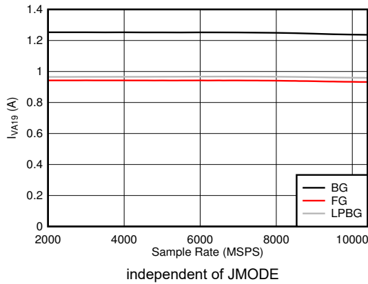
图 5-121. DES Mode: I_{VA19} vs Sample Rate
