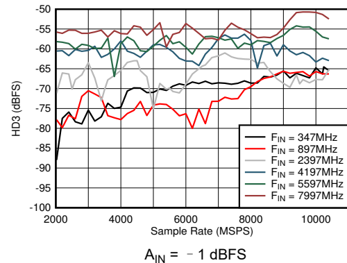
图 5-38. DES Mode: HD3 vs Sample Rate and Input Frequency
