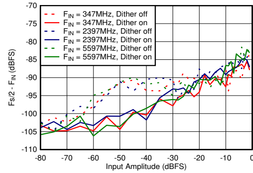
图 5-80. Dual Channel Mode: F_{\text{s}}/2 - F_{\text{IN}} vs Input Amplitude and Dither
