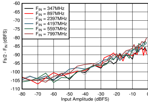
图 5-79. Dual Channel Mode: F_{\text{s}}/2 - F_{\text{IN}} vs Input Amplitude and Frequency
