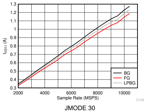
图 5-125. DES Mode: I_{VD11} vs Sample Rate
