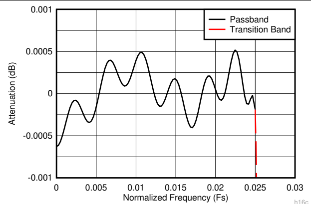
图 6-16. Decimate-by-16 Composite Zoomed Pass-Band Response
