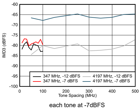
图 6-109. Dual Channel Mode: IMD3 vs Tone Spacing
