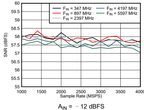
图 6-44. Dual Channel Mode: SNR vs Sample Rate and Input Frequency
