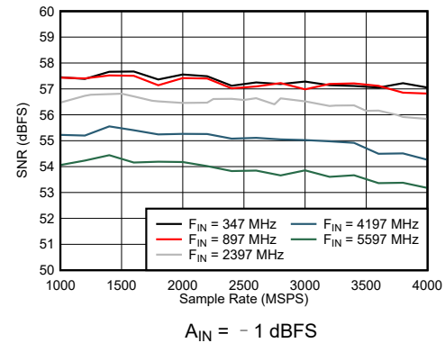
图 6-42. Dual Channel Mode: SNR vs Sample Rate and Input Frequency
