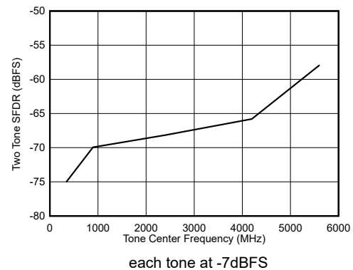
图 6-110. DES Mode: Two Tone SFDR vs Input Frequency
