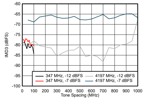
图 6-108. DES Mode: IMD3 vs Tone Spacing
