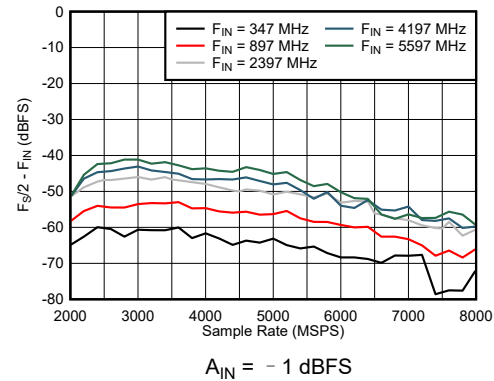
图 6-40. DES Mode: F_S/2 - F_{\text{IN}} vs Sample Rate and Input Frequency
