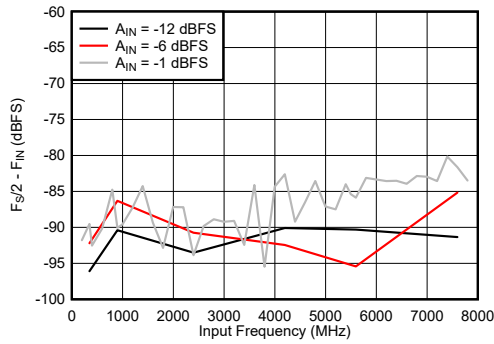
图 6-87. Dual Channel Mode: F_{\text{S}}/2 - F_{\text{IN}} vs Input Frequency
