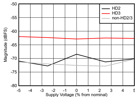
图 6-101. DES Mode: HD2, HD3 and Worst non-HD Spur vs Supply Voltage
