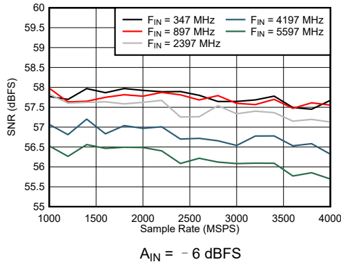
图 6-43. Dual Channel Mode: SNR vs Sample Rate and Input Frequency
