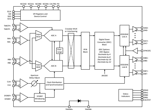
ADC12DJ4000RF 方框图
