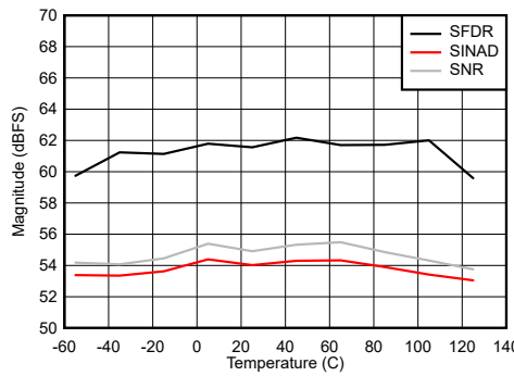
图 6-92. DES Mode: SNR, SINAD and SFDR vs Temperature FG calibration at each temperature
