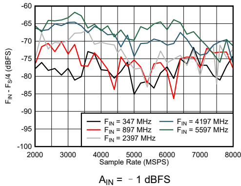
图 6-41. DES Mode: F_{\text{IN}} \pm F_S/4 vs Sample Rate and Input Frequency
