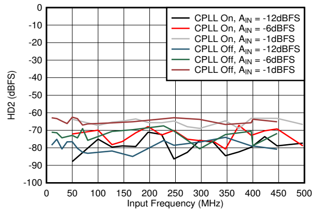
图 6-58. HD2 vs A_{IN} and C-PLL
