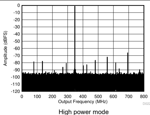
图 6-4. Single Tone FFT at 347 MHz and -1 dBFS
