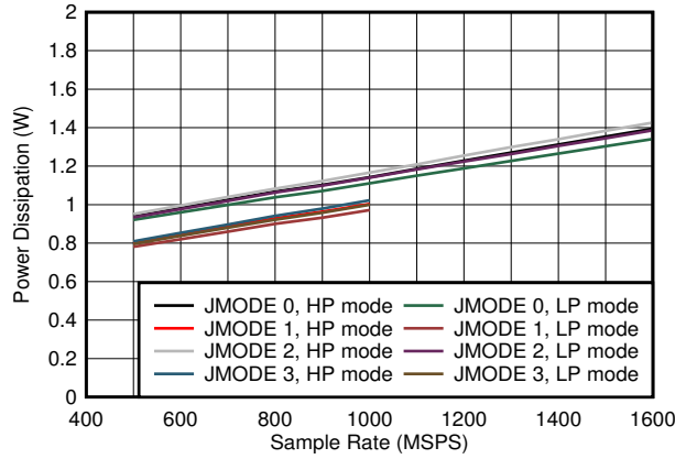
图 6-99. Single Channel, Power Dissipation vs F_S and JMODE 0 - 3
