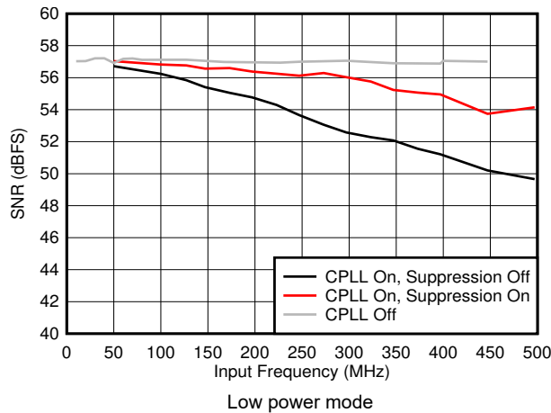
图 6-45. SNR vs F_{IN} and C-PLL modes
