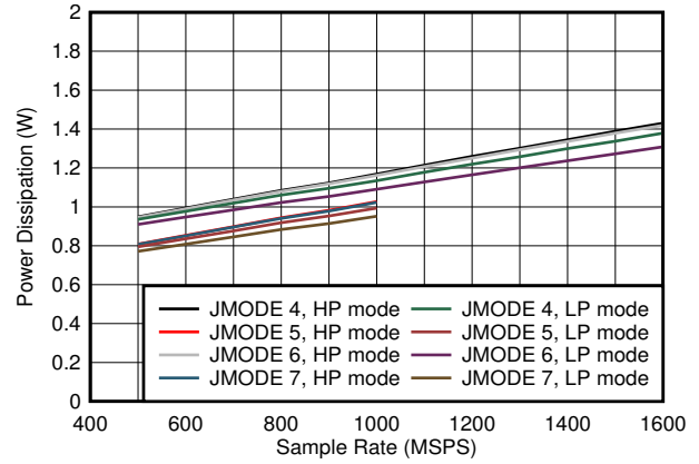
图 6-100. Single Channel, Power Dissipation vs F_S and JMODE 4 - 7
