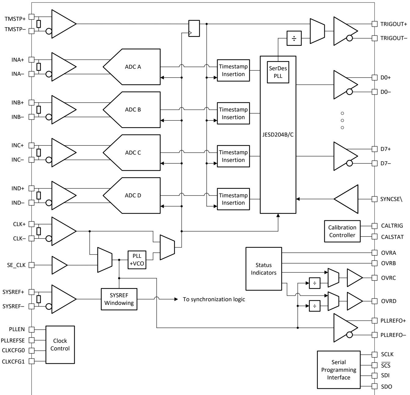
图 7-1. Quad Channel Functional Block Diagram
