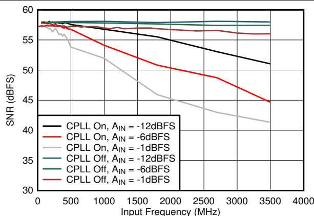
图 6-49. SNR vs A_{IN} and C-PLL
