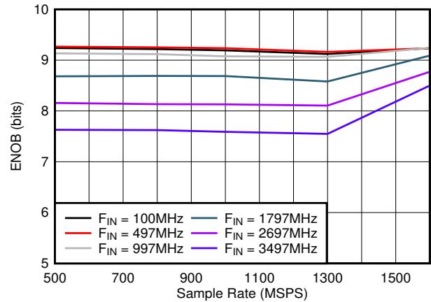
图 6-26. ENOB vs Sample Rate
