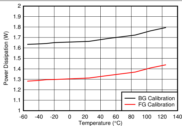
图 6-121. Quad Channel, Power Dissipation vs Temperature
