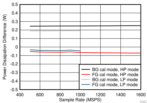
Difference to lower power background calibration, JMODE independent 图 6-111. Single Channel, Power Dissipation Change with Calibration Mode
