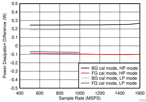
Difference to lower power background calibration, JMODE independent 图 6-109. Quad Channel, Power Dissipation Change with Calibration Mode
