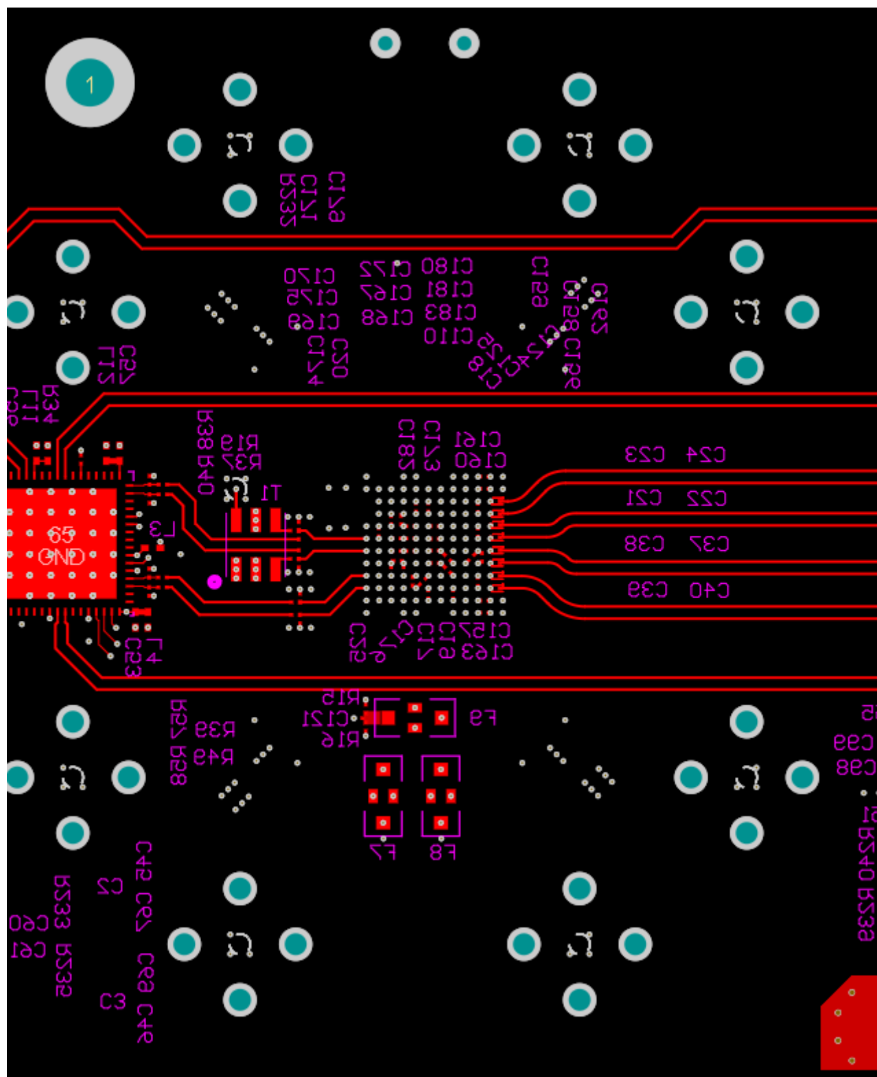
图 8-7. Bottom Layer Routing: CLK±, SYSREF and D[7:4]± Routing
