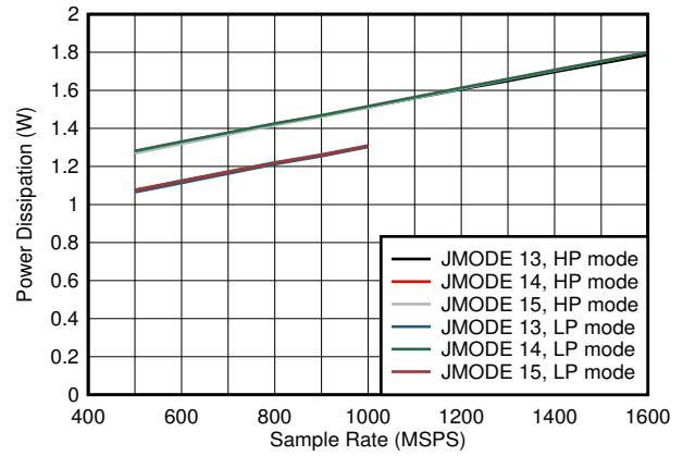
图 6-92. Dual Channel, Power Dissipation vs F_S and JMODE 13 - 15
