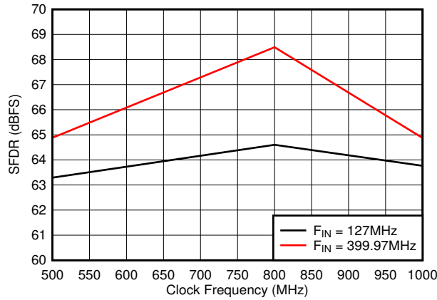
图 6-29. SFDR vs Sample Rate
