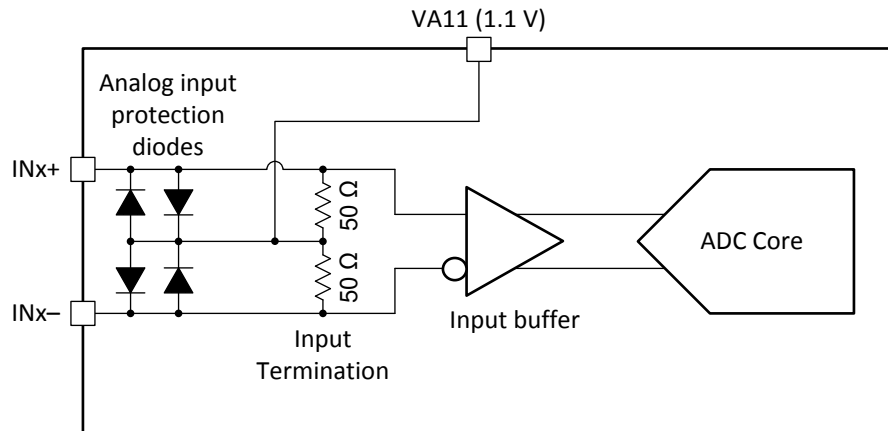
图 7-4. Analog Input Internal Termination and Protection Diagram
