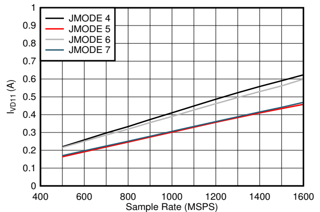
图 6-84. Quad Channel, I_{VDD11} vs F_S
