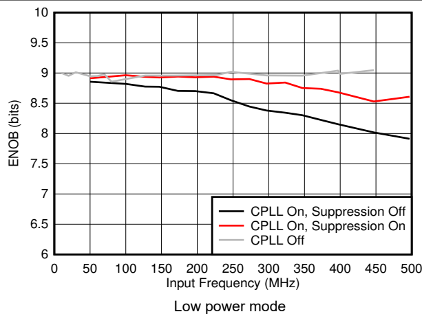
图 6-47. ENOB vs F_{IN} and C-PLL modes
