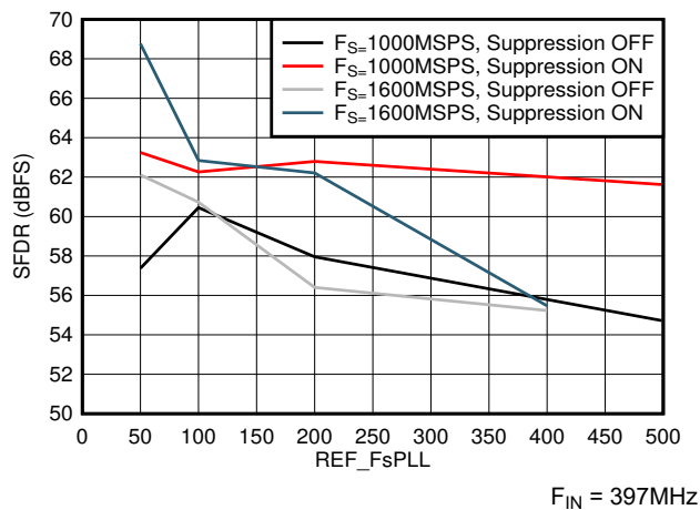
图 6-39. SFDR vs F_{REF} and Suppression
