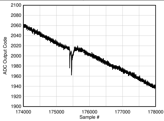
图 6-125. Background Calibration Core Transition (offset voltage)
