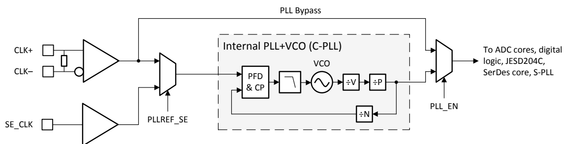
图 7-6. Converter PLL (C-PLL) Architecture
