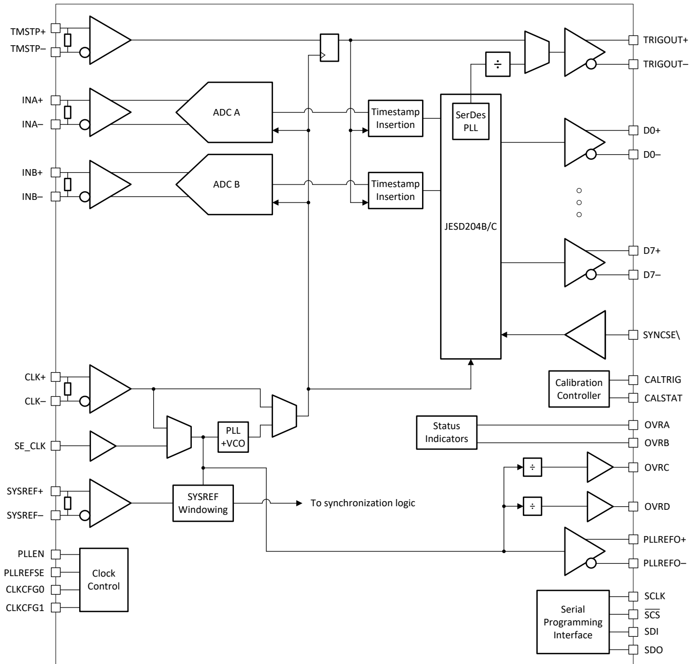
图 7-2. Dual Channel Functional Block Diagram
