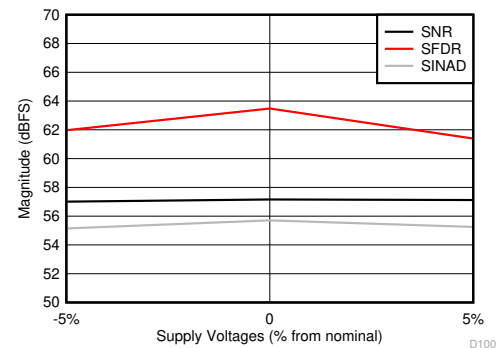
图 6-60. SNR, SFDR and SINAD vs Supply Voltage
