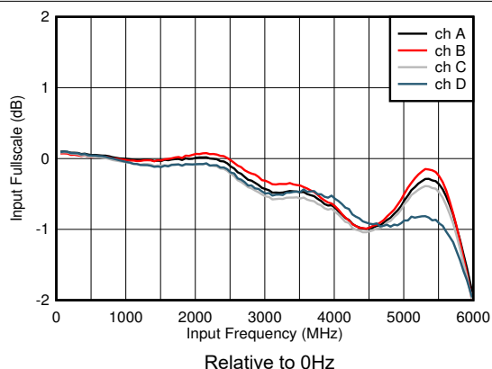
图 6-3. Input Fullscale vs Frequency
