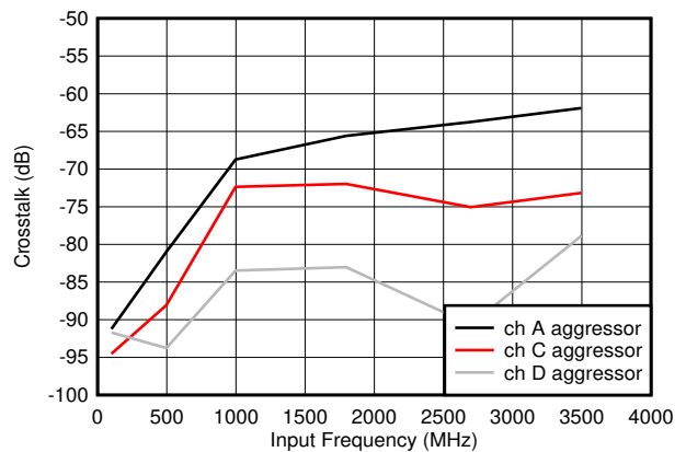
图 6-78. Crosstalk to Channel B vs F_{IN}
