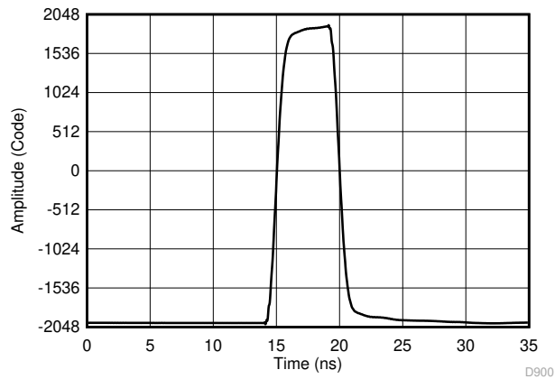
图 8-2. Measured Pulse using Sub-Sampling Technique for Equivalent 32 GSPS Measurement
