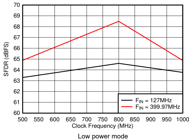
图 6-27. SFDR vs Sample Rate
