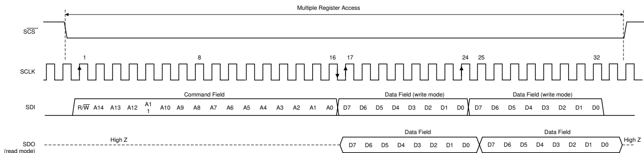
图 7-19. Serial Interface Protocol: Streaming Read/Write
