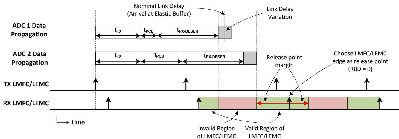
图 7-11. LMFC/LEMC Valid Region Definition for Elastic Buffer Release Point Selection
