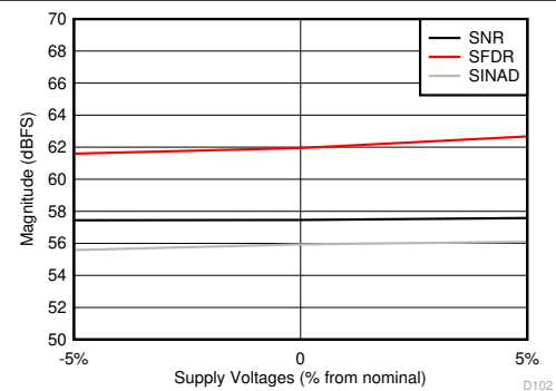
图 6-62. SNR, SFDR and SINAD vs Supply Voltages
