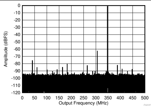
图 6-10. Single Tone FFT at 1797 MHz and -1 dBFS
