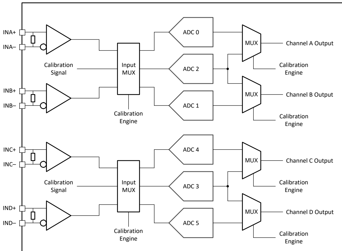
图 7-15. Quad Channel Calibration System Block Diagram
