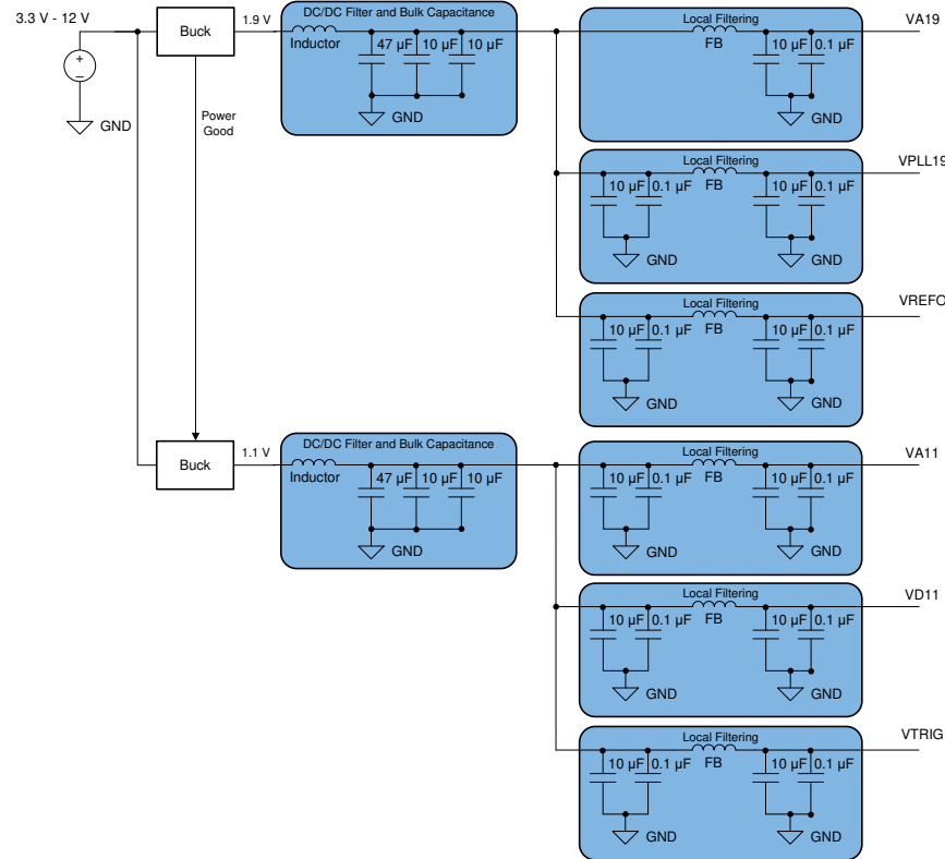
图 8-4. Switcher-Only Approach Example
