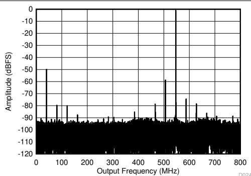
图 6-9. Single Tone FFT at 997 MHz and -1 dBFS
