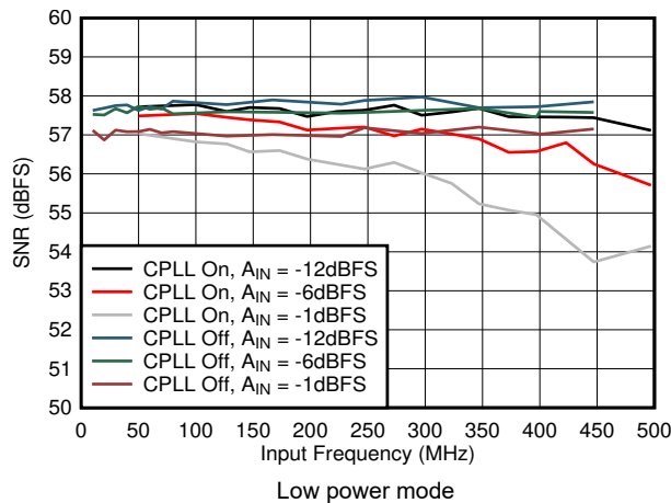
图 6-55. SNR vs A_{IN} and C-PLL
