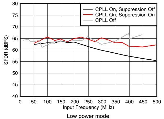
图 6-44. SFDR vs F_{IN} and C-PLL modes
