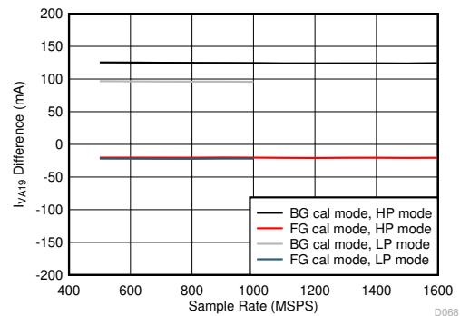
Difference to lower power background calibration, JMODE independent 图 6-112. Quad Channel, I_{VA19} Change with Calibration Mode
