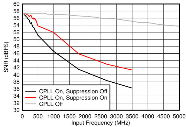
图 6-41. SNR vs F_{IN} and C-PLL modes
