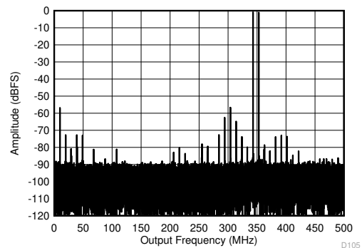
图 6-70. Two Tone FFT at 1798MHz
