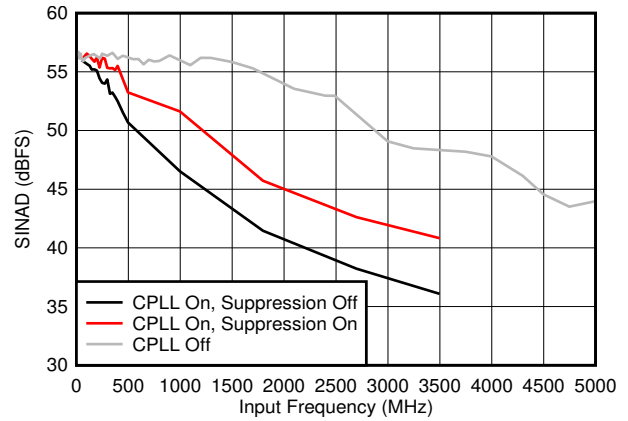
图 6-42. SINAD vs F_{IN} and C-PLL modes
