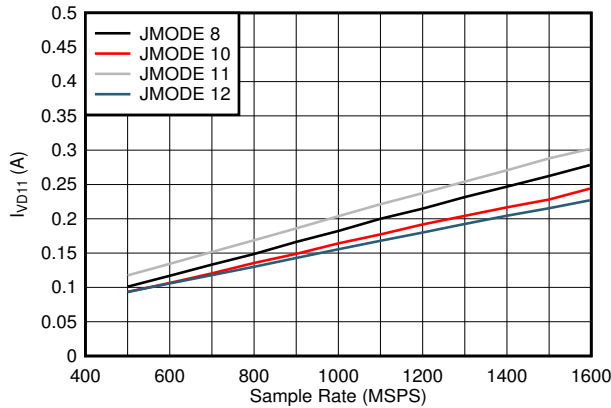
Low power background calibration mode 图 6-107. Single Channel, I_{VD11} vs F_S and JMODE 8 - 12
