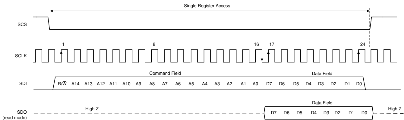
图 7-18. Serial Interface Protocol: Single Read/Write
