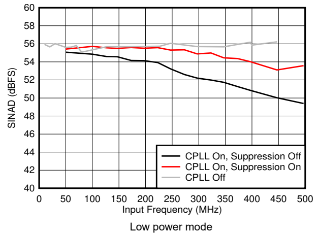
图 6-46. SINAD vs F_{IN} and C-PLL modes
