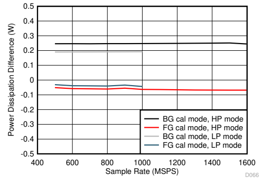
Difference to lower power background calibration, JMODE independent 图 6-110. Dual Channel, Power Dissipation Change with Calibration Mode
