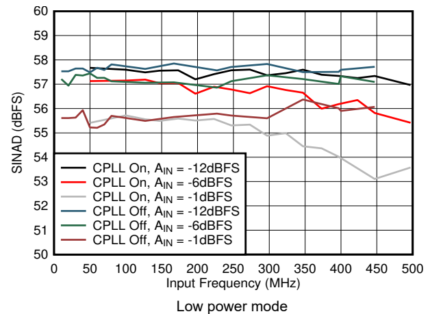
图 6-56. SINAD vs A_{IN} and C-PLL
