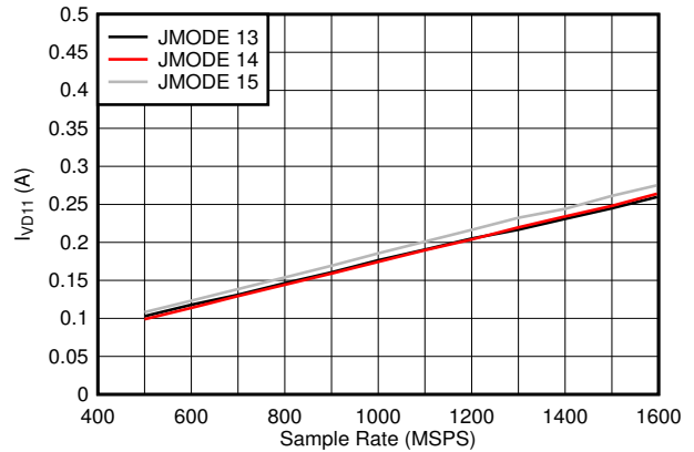
Low power background calibration mode 图 6-108. Single Channel, I_{VD11} vs F_S and JMODE 13 - 15
