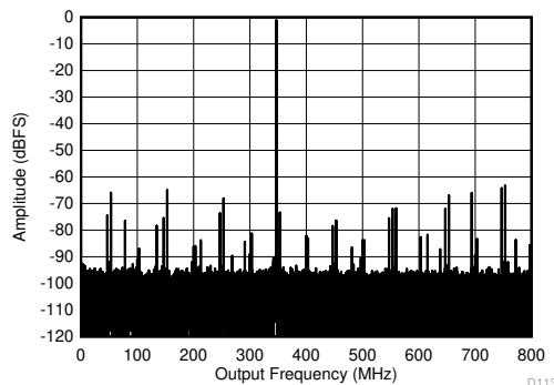
图 6-6. Single Tone FFT at 347 MHz and -1 dBFS
