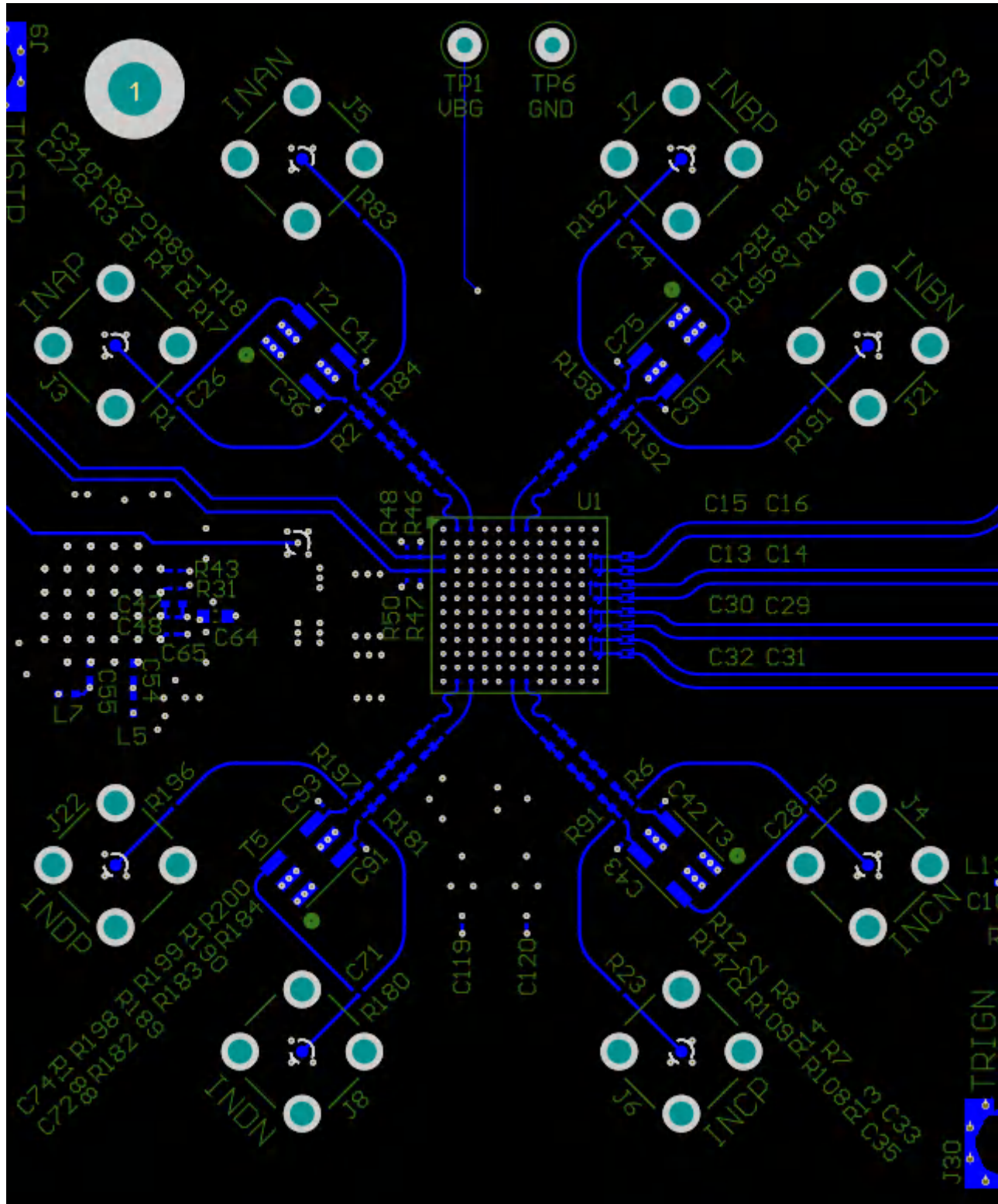
图 8-5. Top Layer Routing: Analog Inputs (INA±, INB±, INC±, IND±), TMSTP± and D[3:0]± Routing
