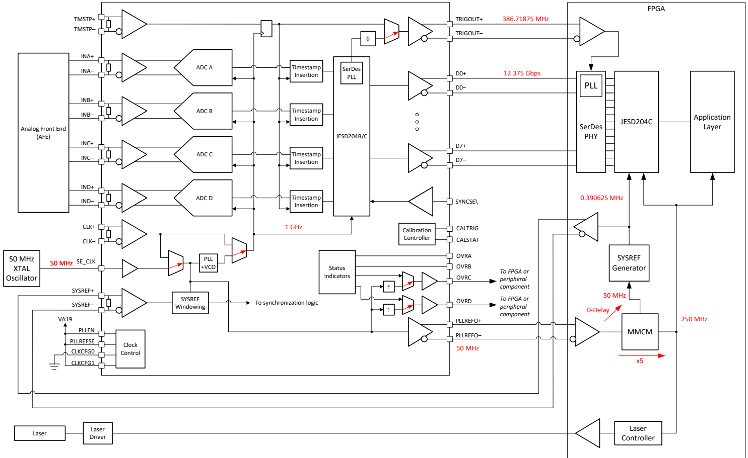
图 8-1. Typical Configuration for a LiDAR Digitizer
