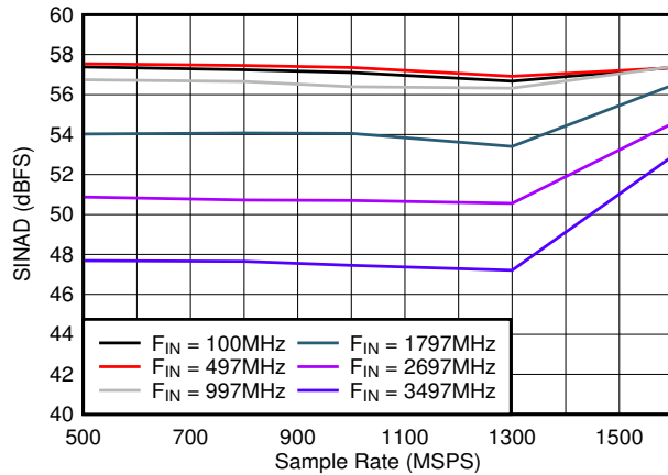
图 6-25. SINAD vs Sample Rate
