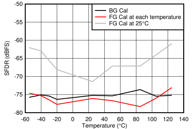
图 6-68. Worst Spur vs Temperature
