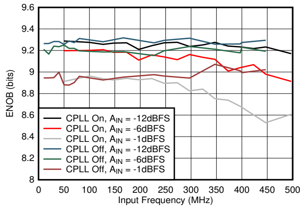
图 6-57. ENOB vs A_{IN} and C-PLL
