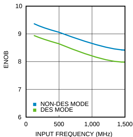
Figure 4-16. ENOB vs. Input Frequency (ADC12D1800)
