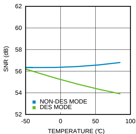
Figure 4-18. SNR vs. Temperature (ADC12D1800)
