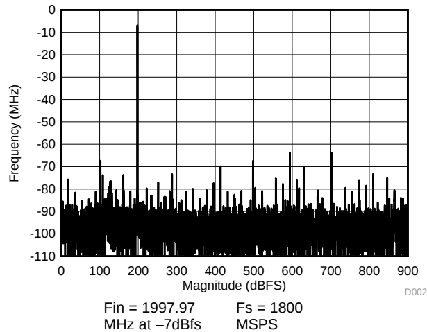
Figure 6-8. Spectrum NON-DES Mode
