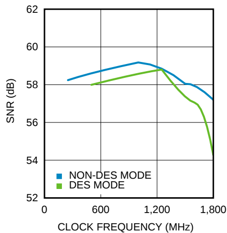
Figure 4-20. SNR vs. Clock Frequency (ADC12D1800)
