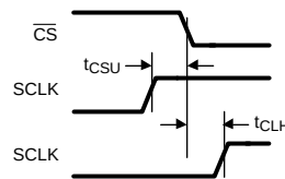
Figure 6. SCLK and \overline{\text{CS}} Timing Parameters
