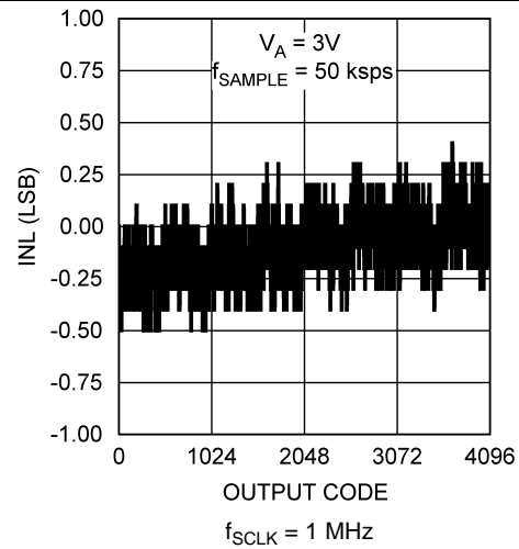
Figure 3. INL
