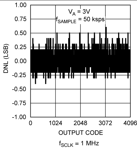
Figure 2. DNL
