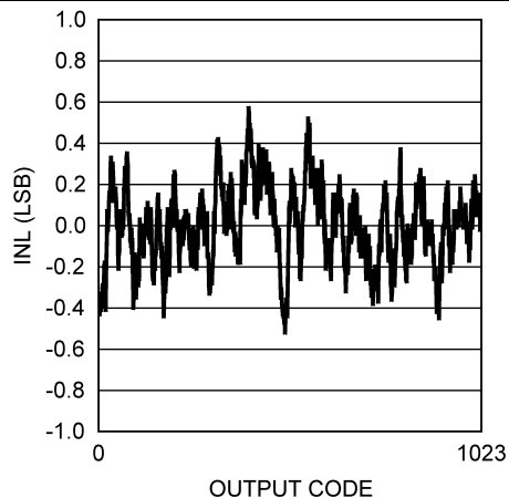
Figure 8. INL vs Code
