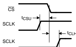
Figure 6. SCLK and CS Timing Parameters
