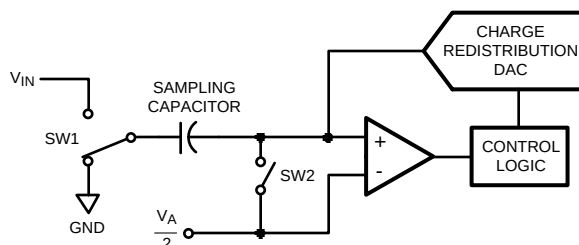
Figure 18. ADC101S101 in Hold Mode
