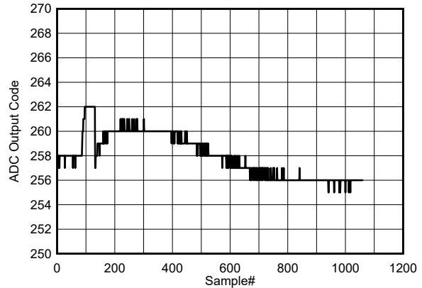
图 5-116. Background Core Transition (DC midscale input)
