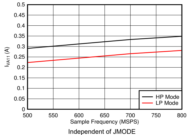
图 5-86. Dual Channel, I_{VA11} vs F_S
