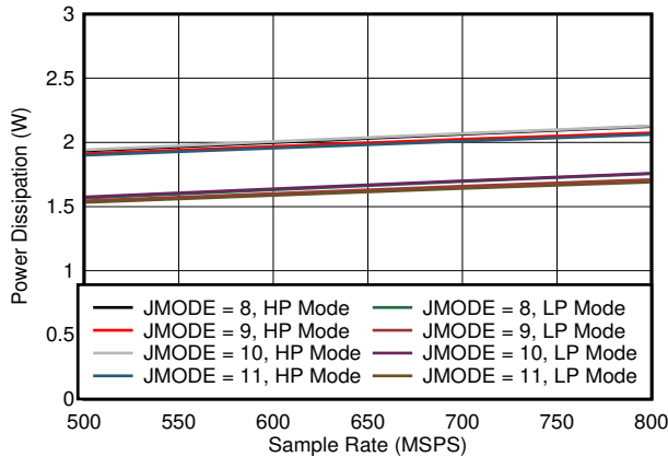
图 5-73. Quad Channel, Power Dissipation vs F_S for JMODES 8 - 11
