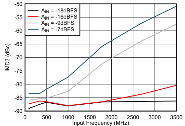
Low Power Mode, 10 MHz Tone Spacing
