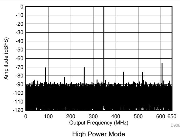
图 5-4. Single Tone FFT at 347 MHz and -1 dBFS
