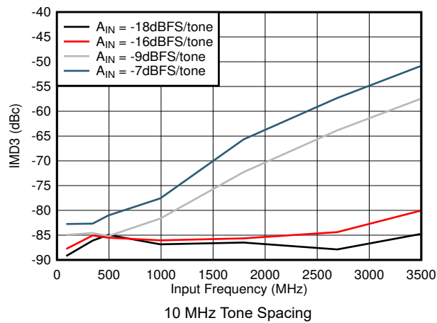
图 5-57. IMD3 vs Input Frequency
