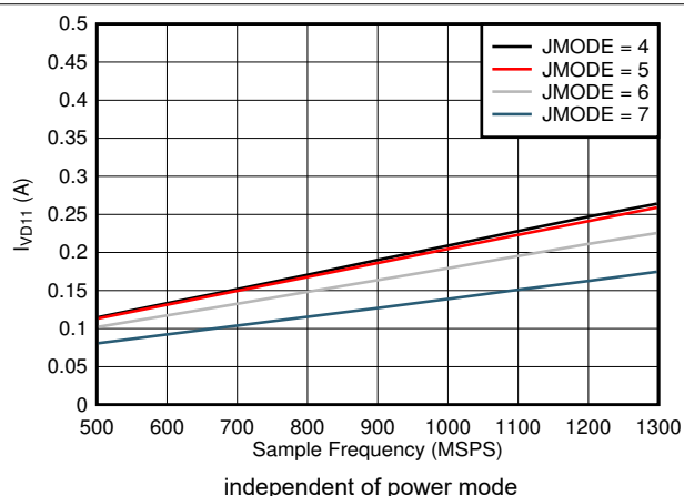
图 5-108. Single Channel, I_{VD11} vs FS and JMODE 4 - 7
