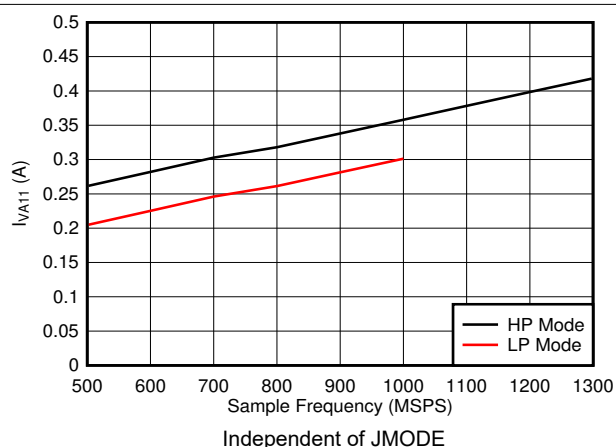
图 5-106. Single Channel, I_{VA11} vs FS
