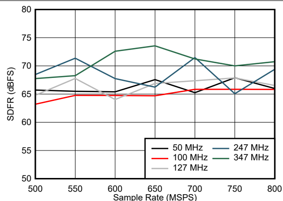
图 5-24. SFDR vs Sample Rate Low Power Mode
