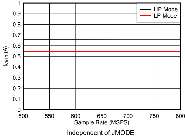
图 5-75. Quad Channel, I_{VA19} vs F_S
