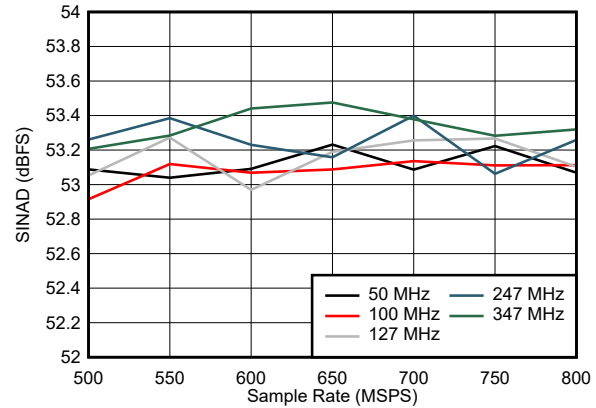
图 5-26. SINAD vs Sample Rate
