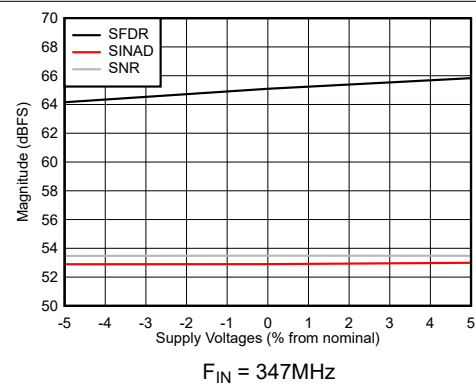
图 5-46. SNR, SFDR and SINAD vs Supply Voltage
