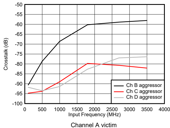
图 5-61. Crosstalk vs Input Frequency
