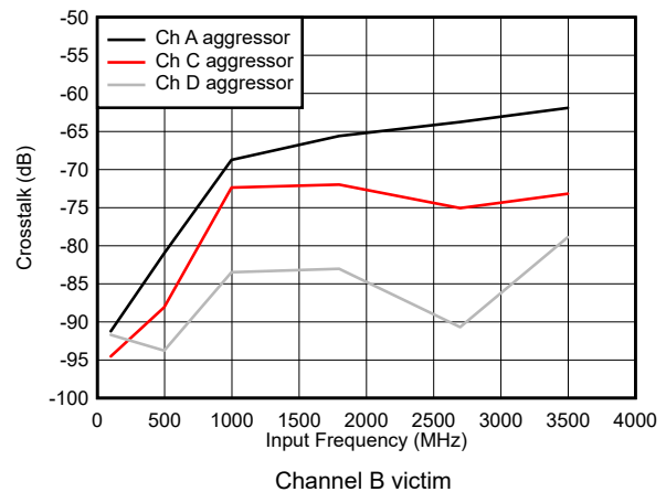
图 5-62. Crosstalk vs Input Frequency
