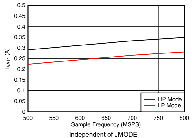
图 5-86. Dual Channel, I_{VA11} vs F_S
