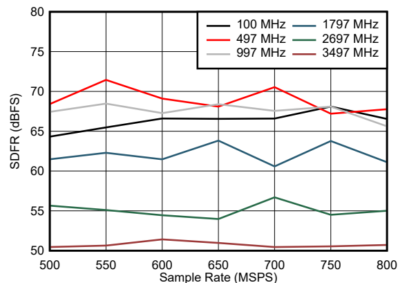
图 5-20. SFDR vs Sample Rate
