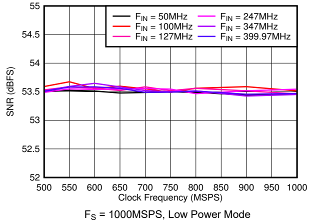
图 5-26. SNR vs Sample Rate
