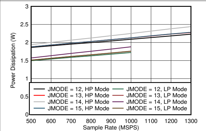
图 5-84. Quad Channel, Power Dissipation vs FS for JMODES 12 - 15
