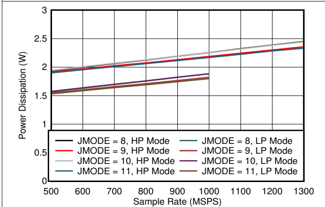
图 5-83. Quad Channel, Power Dissipation vs FS for JMODES 8 - 11
