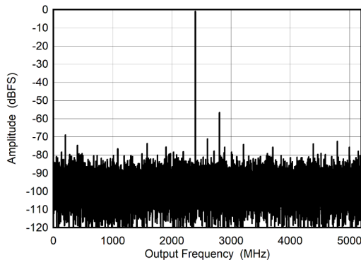
Figure 5-7. DES Mode: Single Tone FFT at 2397 MHz
