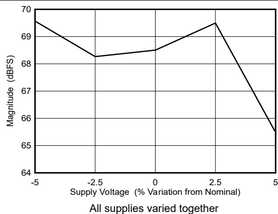
Figure 5-96. Dual Channel Mode: SFDR vs Supply Voltage
