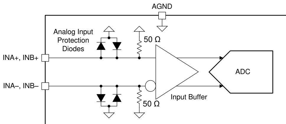
Figure 6-1. ADC08DJ5200RF Analog Input Internal Termination and Protection Diagram
