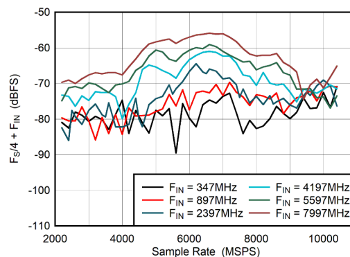
Figure 5-42. DES Mode: F_S/4 + F_{\text{IN}} vs Sample Rate
