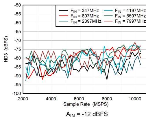
Figure 5-40. DES Mode: HD3 vs Sample Rate
