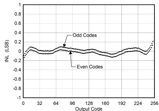
Figure 5-4. INL vs ADC Code
