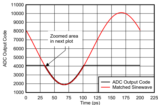
Figure 5-125. Sinewave Overdrive Recovery
