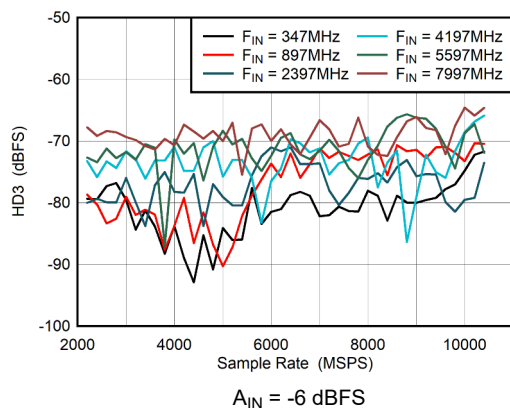
Figure 5-39. DES Mode: HD3 vs Sample Rate
