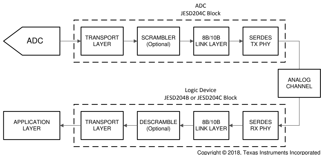
Figure 6-8. Simplified 8B/10B Encoded JESD204C Interface Diagram
