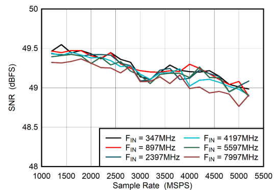
Figure 5-44. Dual Channel Mode: SNR vs Sample Rate
