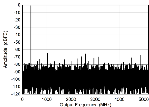
Figure 5-5. DES Mode: Single Tone FFT at 347 MHz
