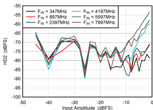
Figure 5-61. DES Mode: HD2 vs Input Amplitude
