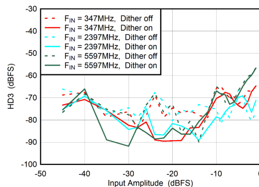
Figure 5-64. DES Mode: HD3 vs Input Amplitude and Dither
