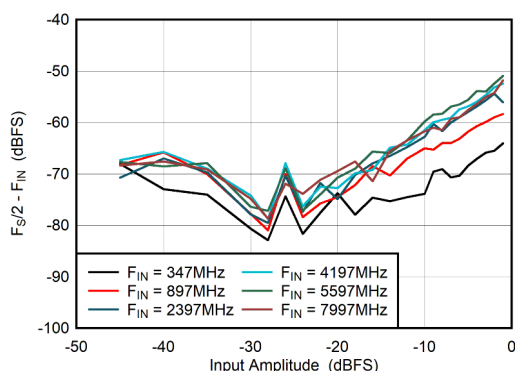
Figure 5-65. DES Mode: F_S/2 - F_{\text{IN}} vs Input Amplitude
