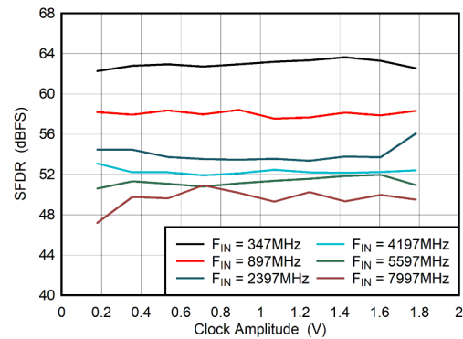
Figure 5-82. DES Mode: SFDR vs Clock Amplitude
