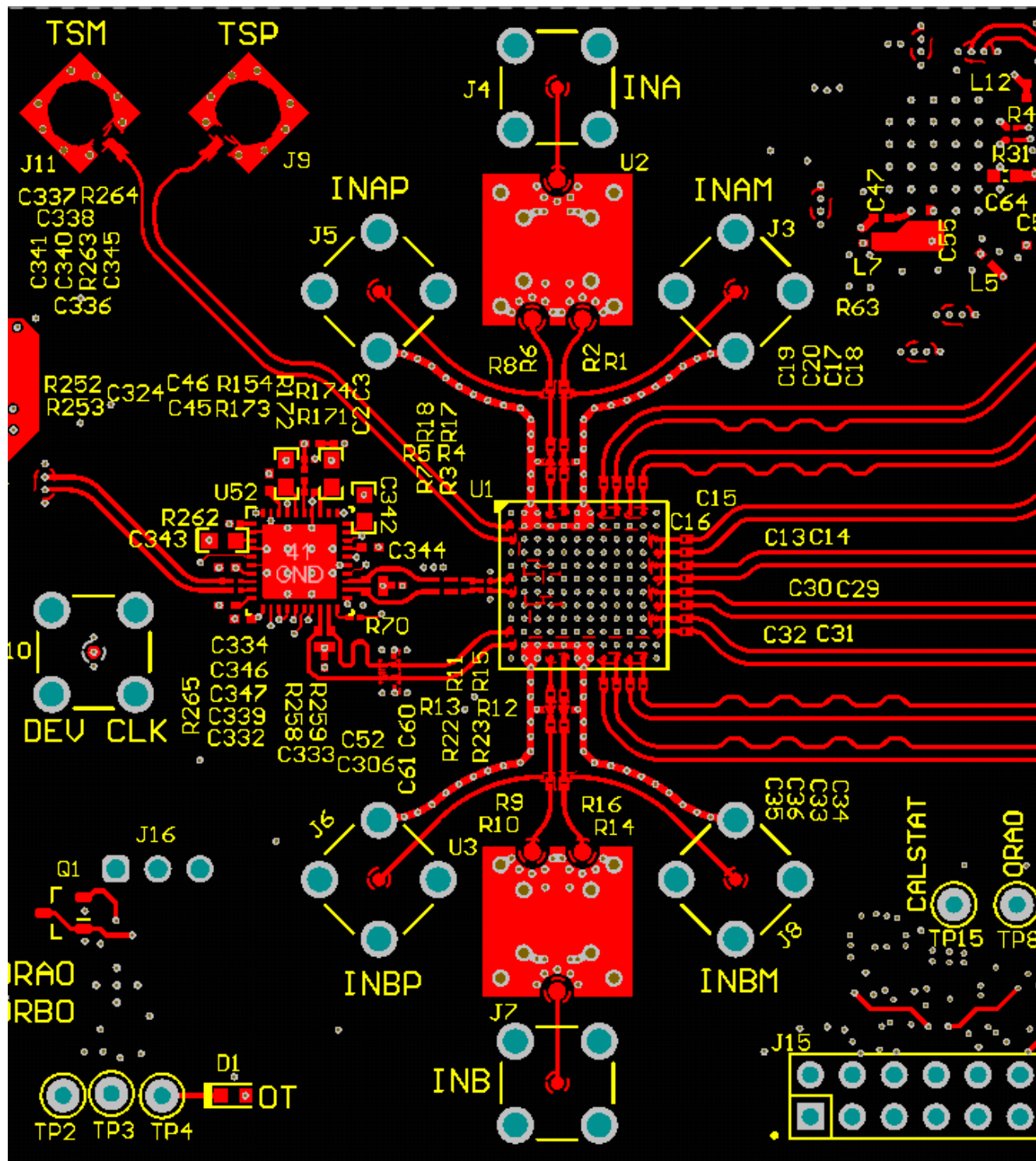
Figure 7-4. Top Layer Routing: Analog Inputs, CLK and SYSREF, DA0-3, DB0-3
