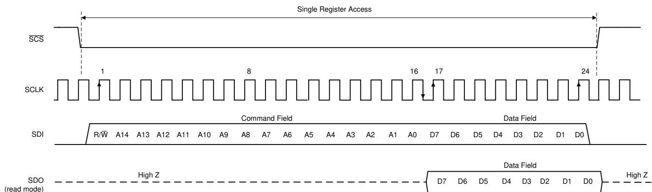
Figure 6-15. Serial Interface Protocol: Single Read/Write
