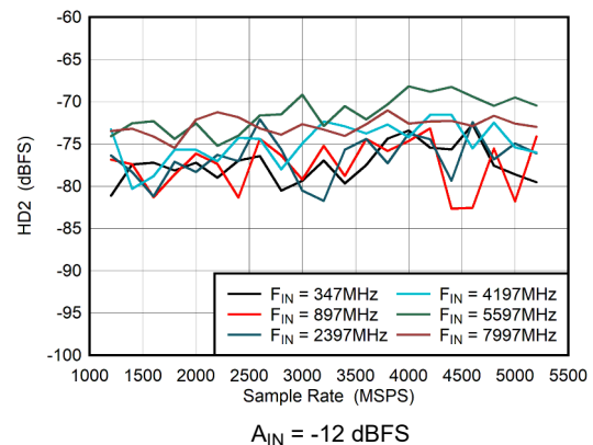
Figure 5-52. Dual Channel Mode: HD2 vs Sample Rate
