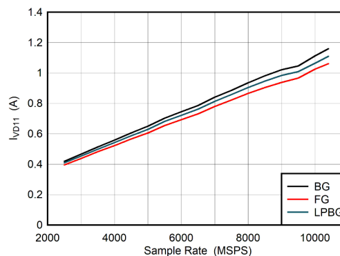
Figure 5-112. DES Mode: I_{VD11} vs Sample Rate
