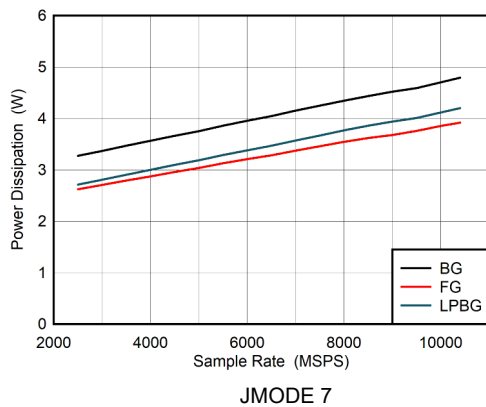
Figure 5-113. DES Mode: Power Dissipation vs Sample Rate
