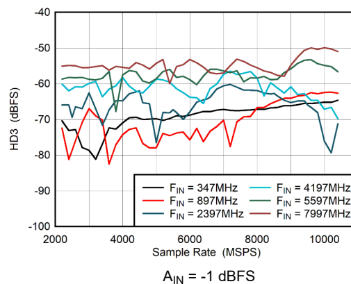
Figure 5-38. DES Mode: HD3 vs Sample Rate
