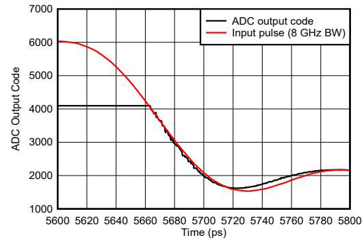
Figure 5-124. Pulse Overdrive Recovery Zoomed
