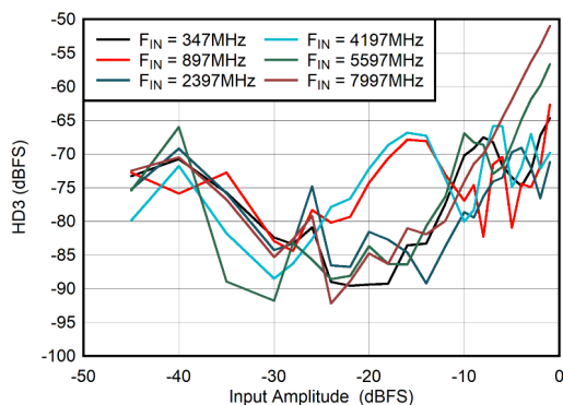
Figure 5-63. DES Mode: HD3 vs Input Amplitude
