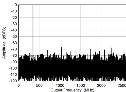
Figure 5-17. Dual Channel Mode: Single Tone FFT at 347 MHz
