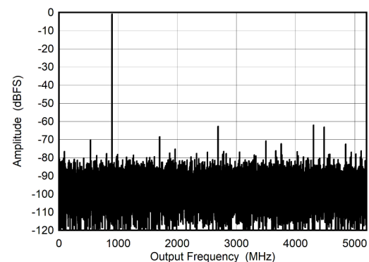
Figure 5-6. DES Mode: Single Tone FFT at 897 MHz
