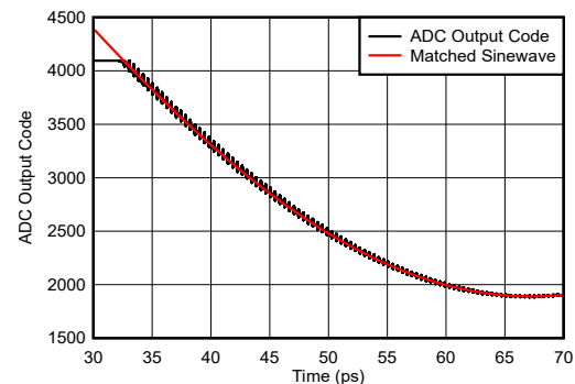
Figure 5-126. Sinewave Overdrive Recovery
