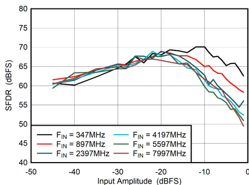
Figure 5-59. DES Mode: SFDR vs Input Amplitude
