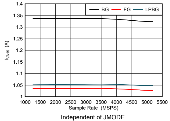
Figure 5-114. Dual Channel Mode: I_{VA19} vs Sample Rate
