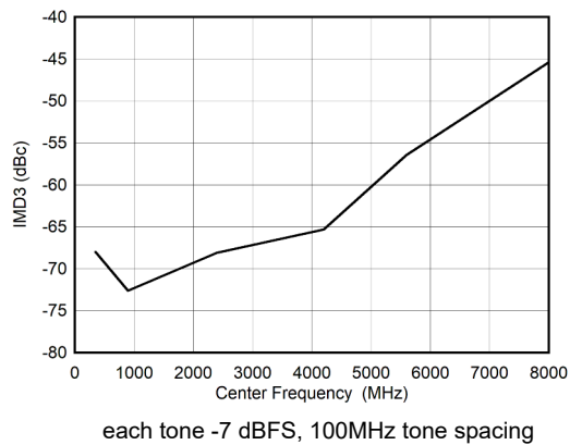
Figure 5-105. Dual Channel Mode: IMD3 vs Input Frequency
