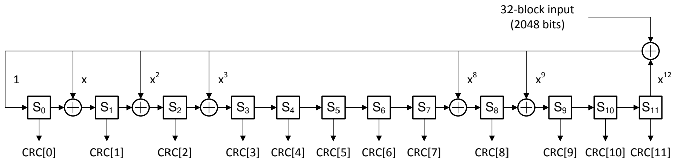
Figure 6-10. CRC-12 Parity Bit Generator
