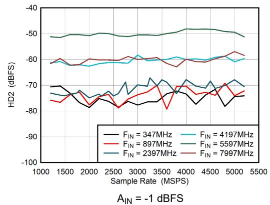
Figure 5-50. Dual Channel Mode: HD2 vs Sample Rate
