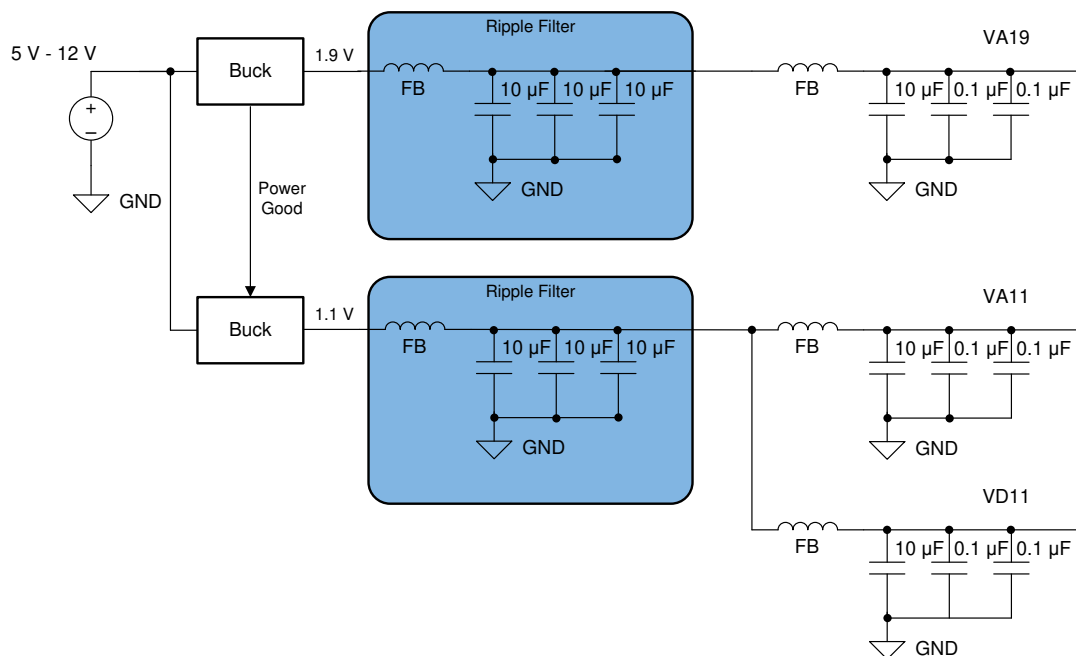
Figure 7-2. LDO Linear Regulator Approach Example
