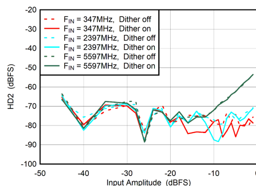
Figure 5-62. DES Mode: HD2 vs Input Amplitude and Dither
