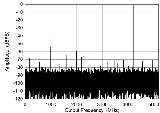
Figure 5-8. DES Mode: Single Tone FFT at 4197 MHz
