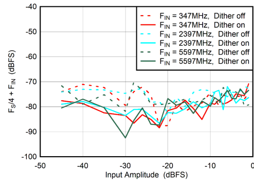
Figure 5-68. DES Mode: F_S/4 + F_{\text{IN}} vs Input Amplitude and Dither
