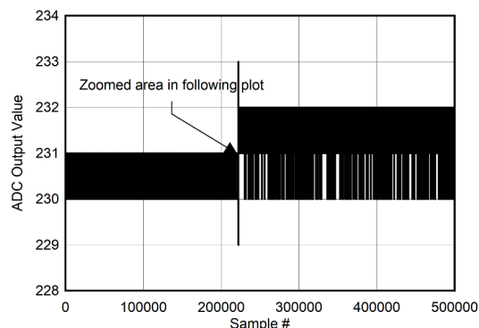
Figure 5-121. Background Calibration Core Transition (DC Signal)
