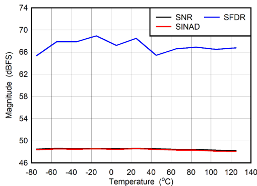
Figure 5-89. Dual Channel Mode: SNR, SINAD and SFDR vs Temperature
