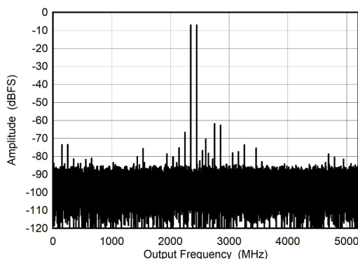
Figure 5-13. DES Mode: Two Tone FFT at 2397 MHz
