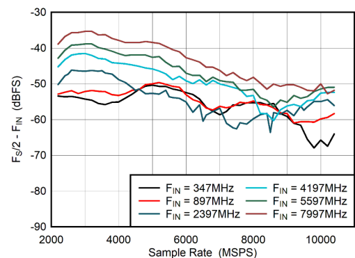
Figure 5-41. DES Mode: F_S/2 - F_{\text{IN}} vs Sample Rate
