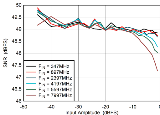
Figure 5-71. Dual Channel Mode: SNR vs Input Amplitude
