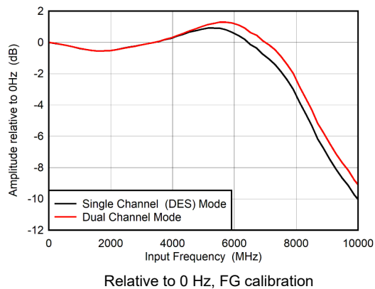
Figure 5-1. Input Amplitude vs Input Frequency
