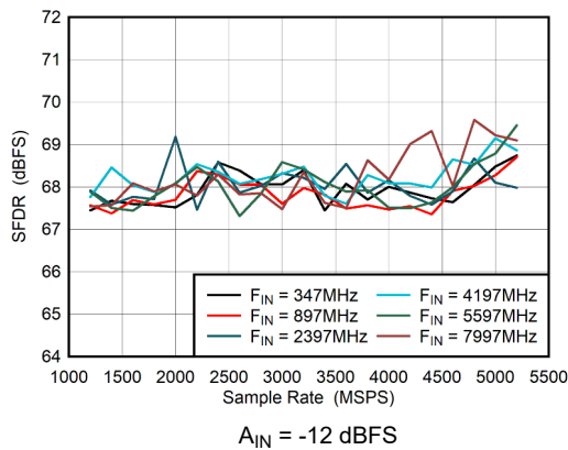
Figure 5-49. Dual Channel Mode: SFDR vs Sample Rate
