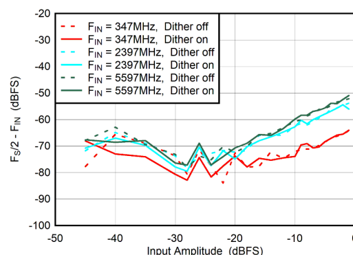
Figure 5-66. DES Mode: F_S/2 - F_{\text{IN}} vs Input Amplitude and Dither
