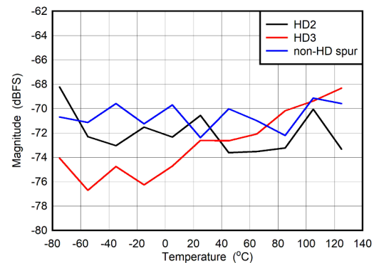
Figure 5-90. Dual Channel Mode: HD2, HD3 and Worst Spur vs Temperature
