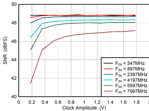
Figure 5-81. DES Mode: SNR vs Clock Amplitude
