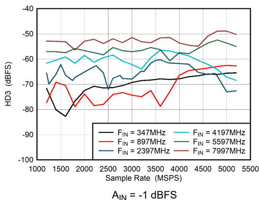
Figure 5-53. Dual Channel Mode: HD3 vs Sample Rate
