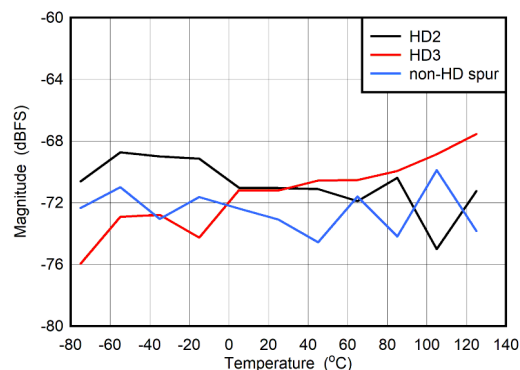
Figure 5-86. DES Mode: HD2, HD3 and Worst Spur vs Temperature
