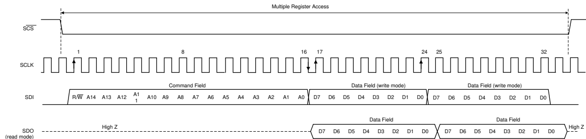
Figure 6-16. Serial Interface Protocol: Streaming Read/Write
