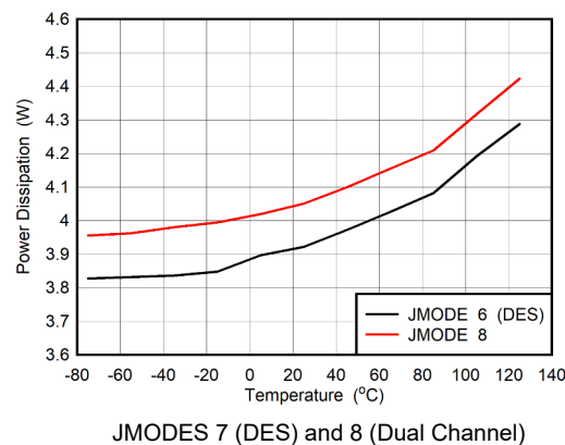
Figure 5-118. Power Dissipation vs Temperature
