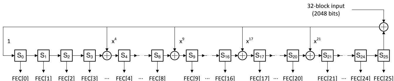
Figure 6-11. FEC Parity Bit Generator
