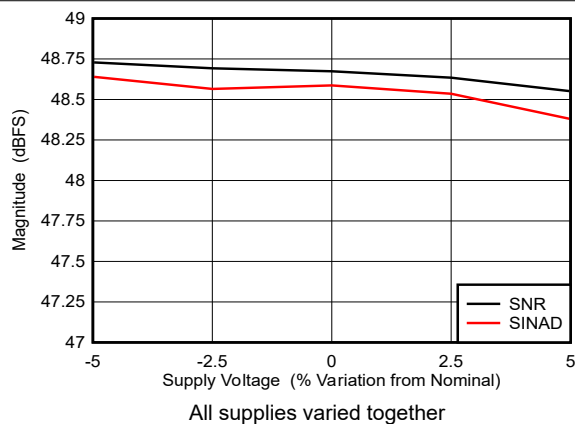
Figure 5-95. Dual Channel Mode: SNR and SINAD vs Supply Voltage
