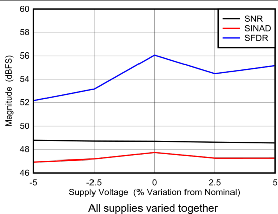
Figure 5-93. DES Mode: SNR, SINAD and SFDR vs Supply Voltage
