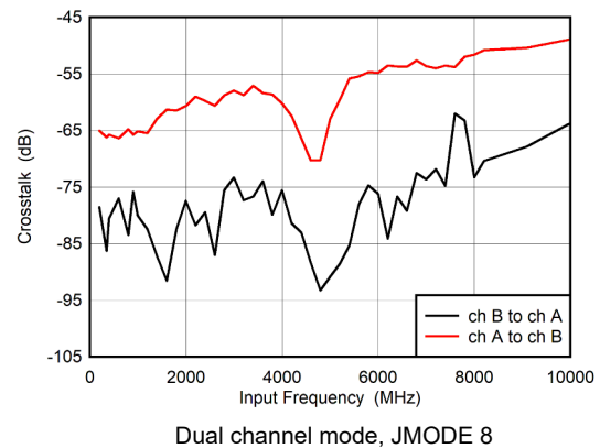
Figure 5-2. Crosstalk vs Input Frequency
