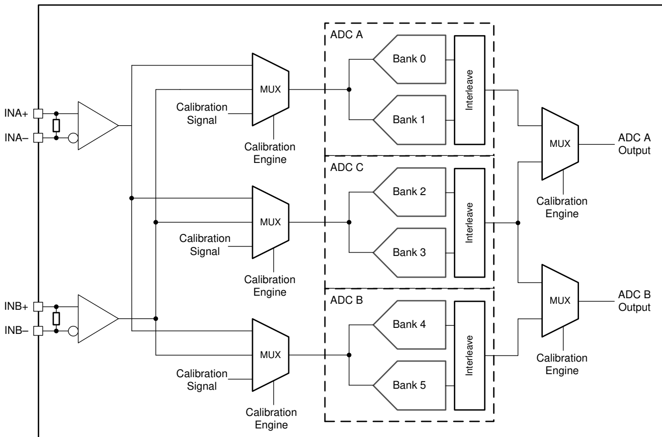
Figure 6-14. ADC08DJ5200RF Calibration System Block Diagram
