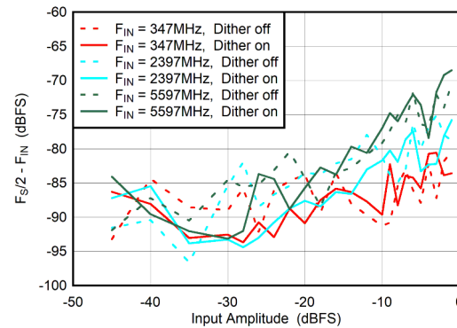
Figure 5-80. Dual Channel Mode: F_S/2 - F_{\text{IN}} vs Input Amplitude and Dither
