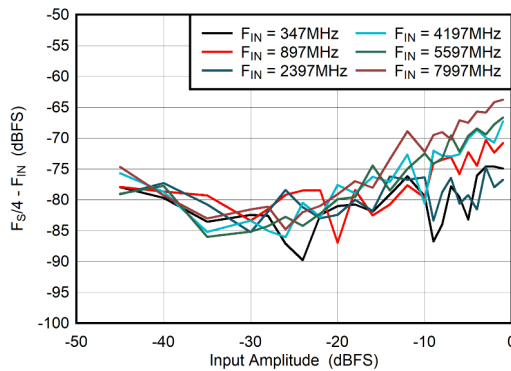
Figure 5-69. DES Mode: F_S/4 - F_{\text{IN}} vs Input Amplitude
