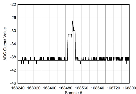
Figure 5-120. Background Calibration Core Transition (AC Signal Zoomed)
