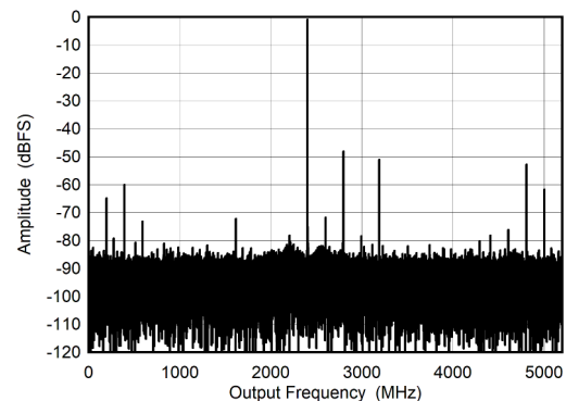
Figure 5-10. DES Mode: Single Tone FFT at 7997 MHz
