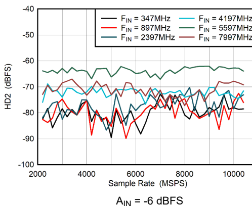
Figure 5-36. DES Mode: HD2 vs Sample Rate
