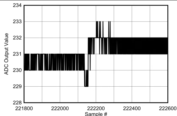
Figure 5-122. Background Calibration Core Transition (DC Signal Zoomed)
