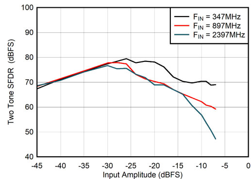
Figure 5-104. DES Mode: Two Tone SFDR vs Input Amplitude
