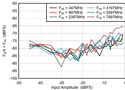
Figure 5-67. DES Mode: F_S/4 + F_{\text{IN}} vs Input Amplitude
