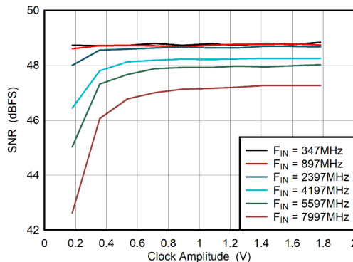
Figure 5-83. Dual Channel Mode: SNR vs Clock Amplitude
