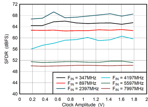
Figure 5-84. Dual Channel Mode: SFDR vs Clock Amplitude
