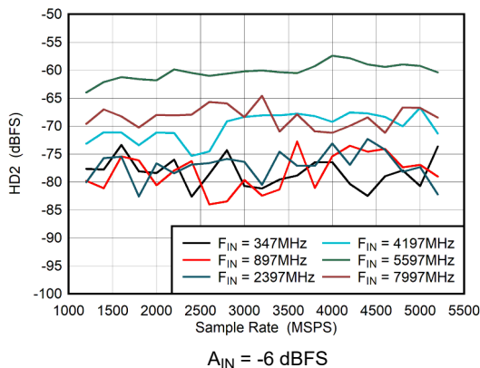
Figure 5-51. Dual Channel Mode: HD2 vs Sample Rate
