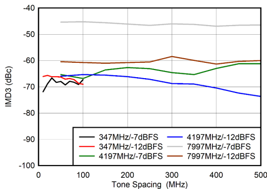
Figure 5-107. Dual Channel Mode: IMD3 vs Tone Spacing
