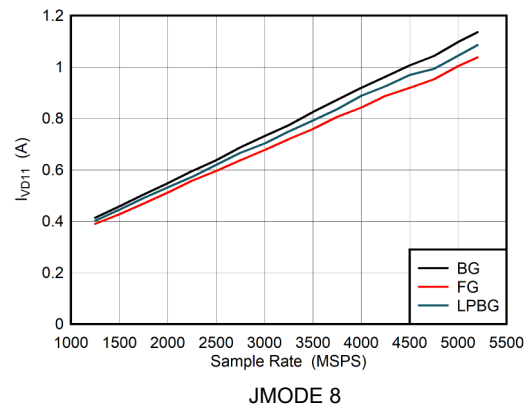
Figure 5-116. Dual Channel Mode: I_{VD11} vs Sample Rate
