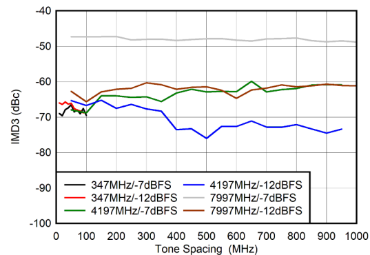
Figure 5-102. DES Mode: IMD3 vs Tone Spacing
