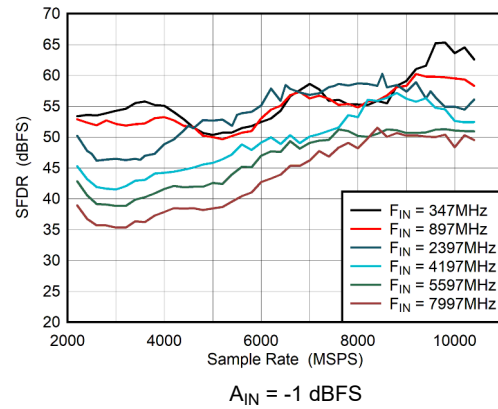
Figure 5-32. DES Mode: SFDR vs Sample Rate
