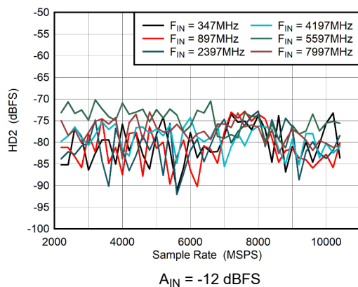
Figure 5-37. DES Mode: HD2 vs Sample Rate
