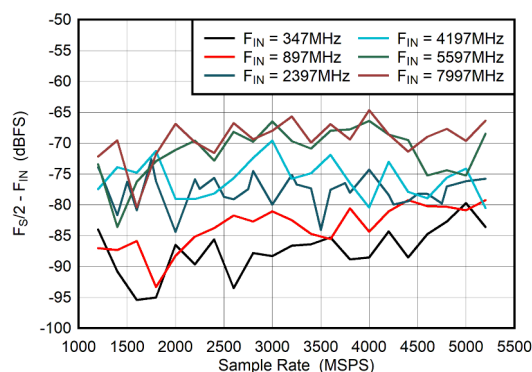
Figure 5-56. Dual Channel Mode: F_{\text{S}}/2 - F_{\text{IN}} vs Sample Rate
