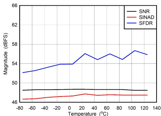
Figure 5-85. DES Mode: SNR, SINAD and SFDR vs Temperature
