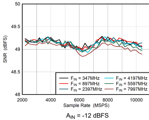
Figure 5-31. DES Mode: SNR vs Sample Rate
