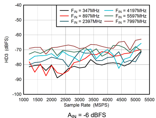
Figure 5-54. Dual Channel Mode: HD3 vs Sample Rate
