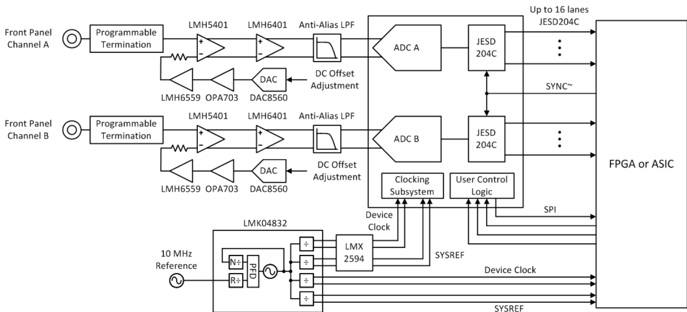
Figure 7-1. Typical Configuration for Reconfigurable Oscilloscope
