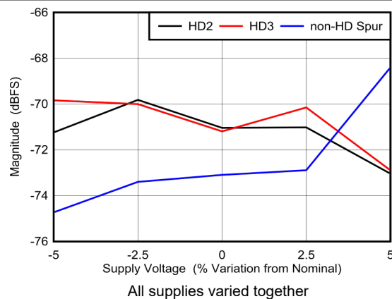
Figure 5-94. DES Mode: HD2, HD3 and Worst Spur vs Supply Voltage
