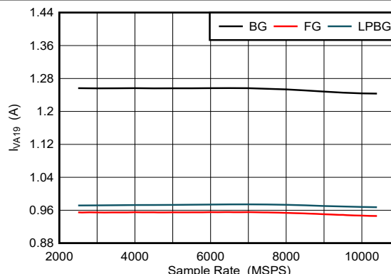
Figure 5-110. DES Mode: I_{VA19} vs Sample Rate
