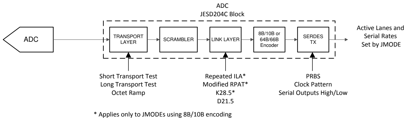
Figure 6-13. Test Mode Insertion Points
