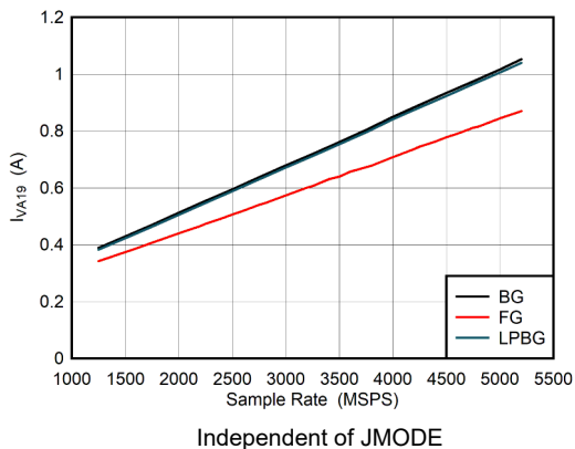
Figure 5-115. Dual Channel Mode: I_{VA11} vs Sample Rate
