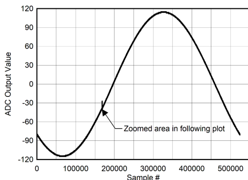
Figure 5-119. Background Calibration Core Transition (AC Signal)
