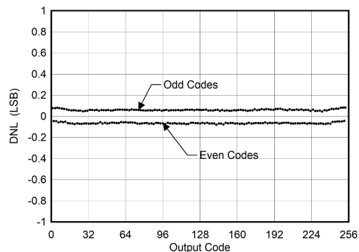
Figure 5-3. DNL vs ADC Code
