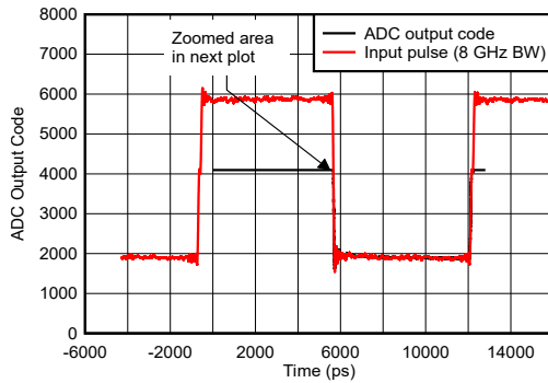
Figure 5-123. Pulse Overdrive Recovery
