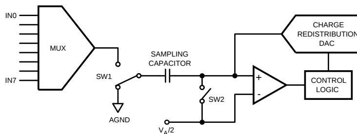
Figure 35. ADC088S022 in Hold Mode
