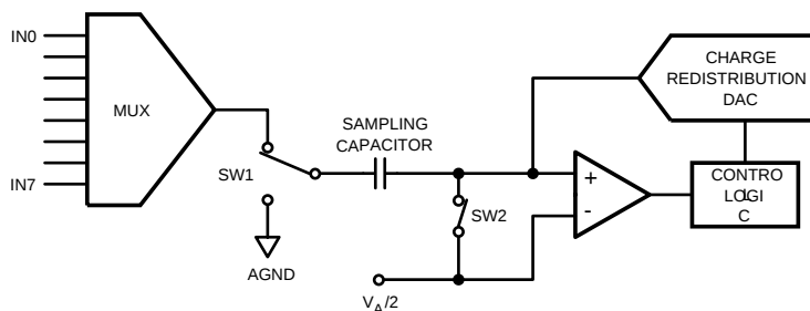
Figure 34. ADC088S022 in Track Mode
