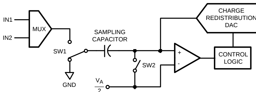
Figure 49. ADC082S101 in Hold Mode
