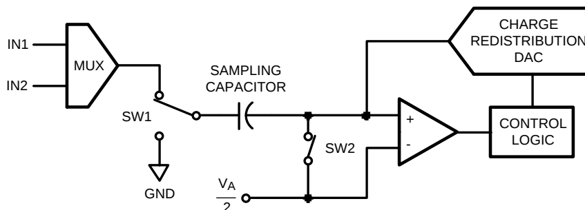
Figure 48. ADC082S101 in Track Mode
