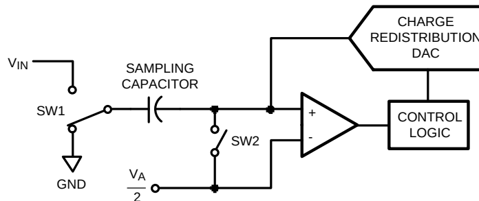
Figure 19. ADC081S051 in Hold Mode
