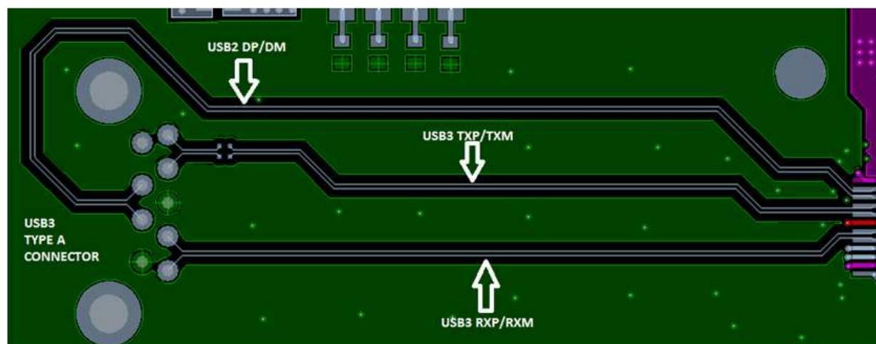
图 47. Example Routing of Downstream Port
