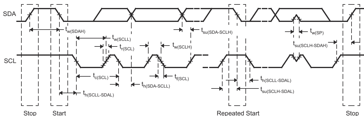
图 8-19. I2C Timings
