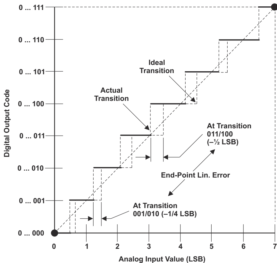
图 8-13. Integral Nonlinearity (INL) Error (A)
