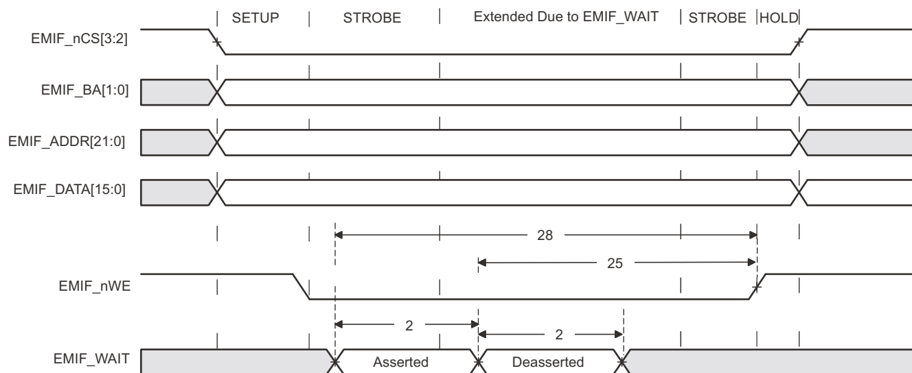
图 7-14. EMIFnWAIT Write Timing Requirements
