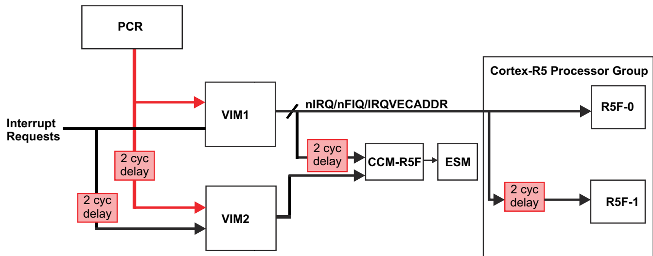
图 7-17. Interrupt Generation
