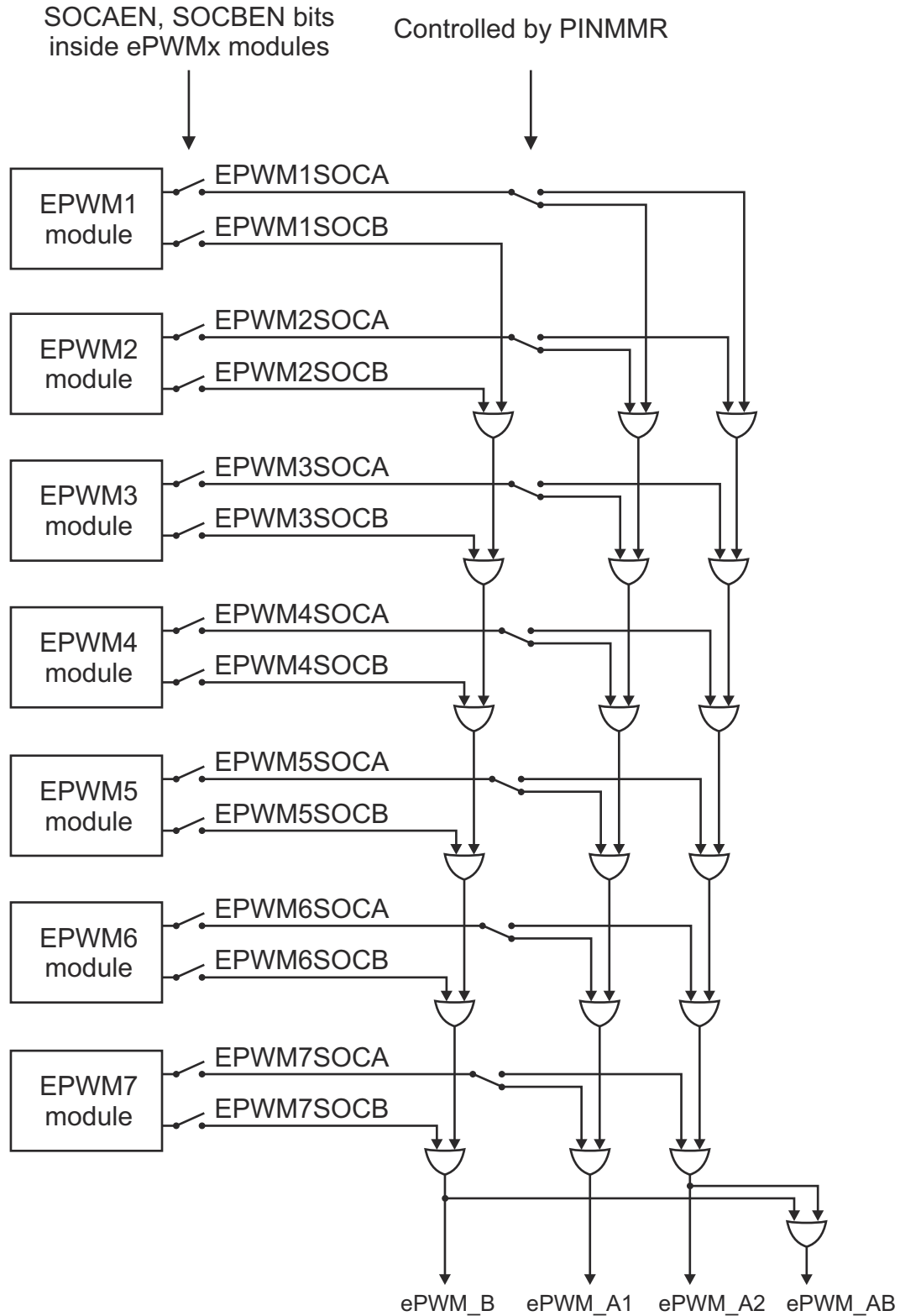
图 8-9. ADC Trigger Source Generation from ePWMx
