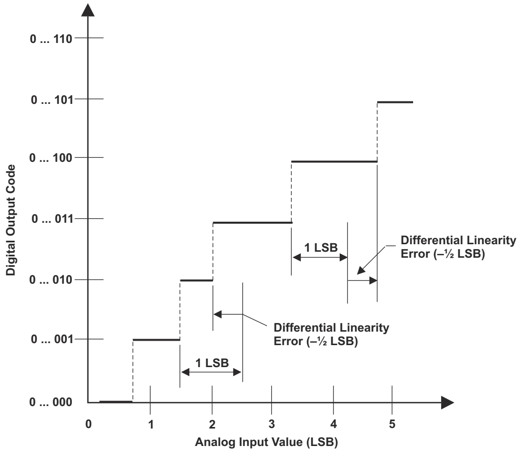
图 8-12. Differential Nonlinearity (DNL) Error
