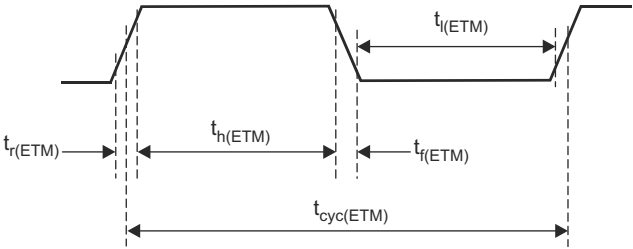
图 7-30. ETMTRACECLKOUT Timing
