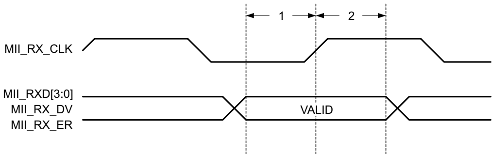
图 8-28. MII Receive Timing
