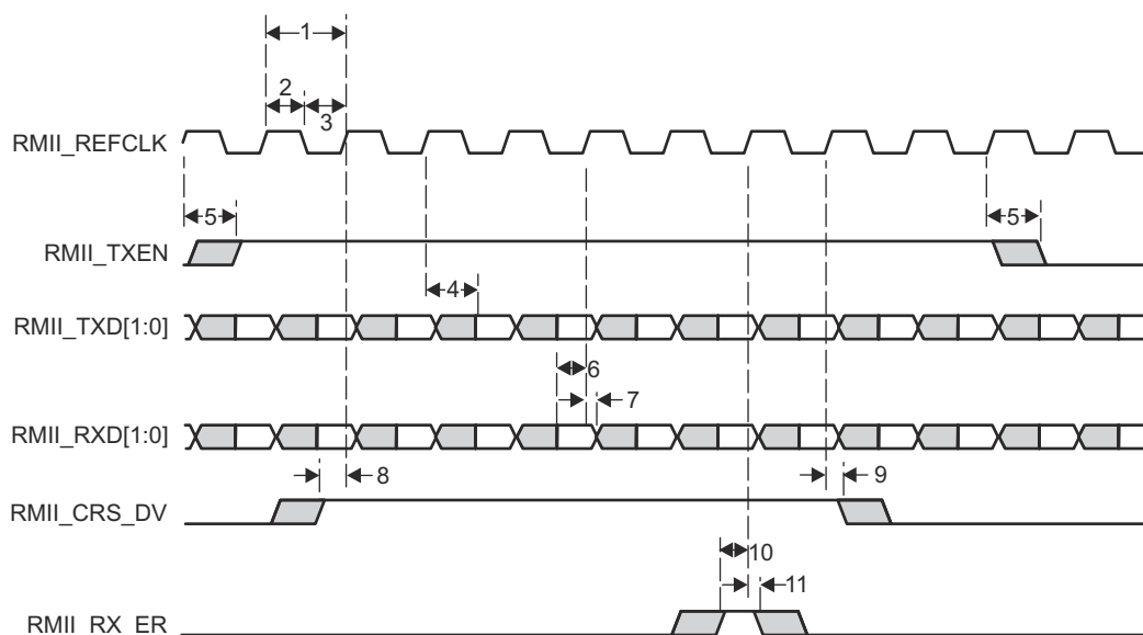
图 8-30. RMII Timing Diagram
