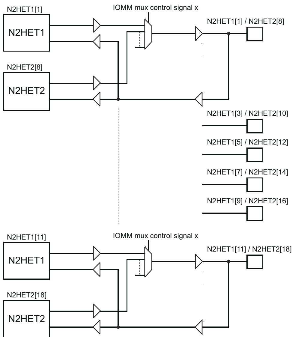
图 8-17. N2HET Monitoring
