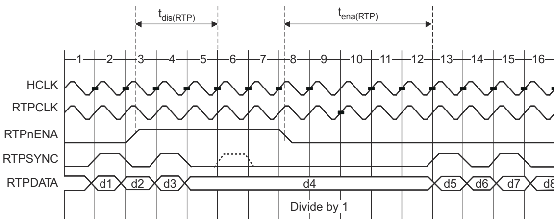
图 7-34. RTPnENA timing
