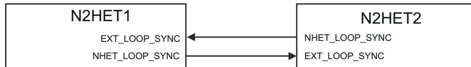
图 8-16. N2HET1 – N2HET2 Synchronization Hookup
