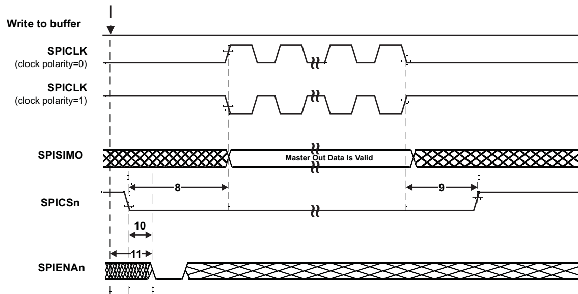
图 7-22. SPI Master Mode Chip Select Timing (CLOCK PHASE = 1)
