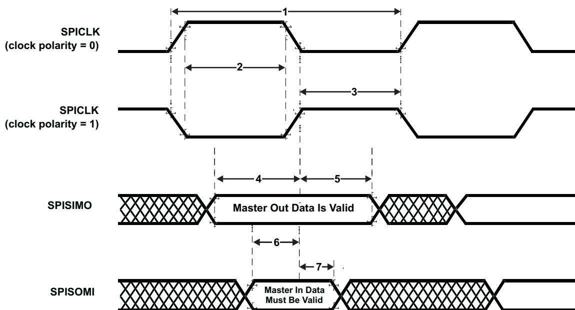
图 7-18. SPI Master Mode External Timing (CLOCK PHASE = 0)
