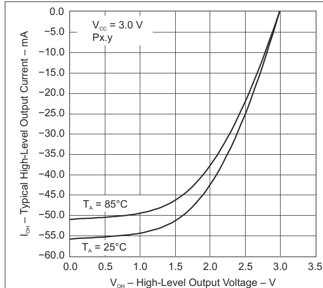
图 7-9. Typical High-Level Output Current vs High-Level Output Voltage
