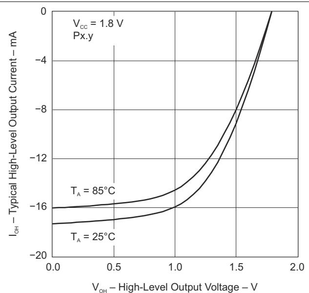
图 7-10. Typical High-Level Output Current vs High-Level Output Voltage
