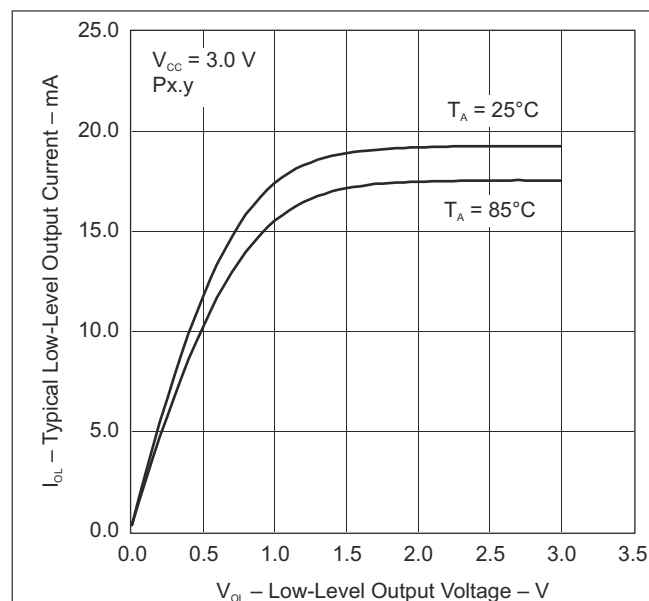
图 7-3. Typical Low-Level Output Current vs Low-Level Output Voltage
