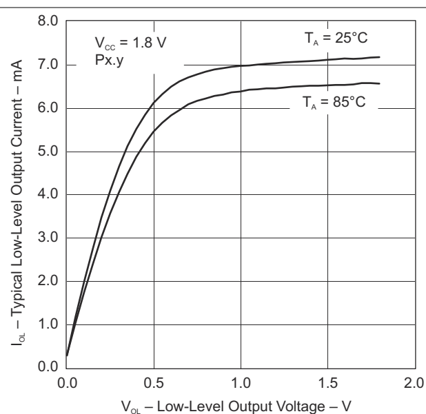
图 7-4. Typical Low-Level Output Current vs Low-Level Output Voltage
