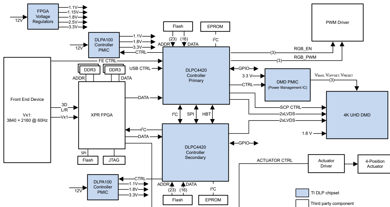
图 7-1. Typical DLPC4420 4K UHD LED Illumination Application
