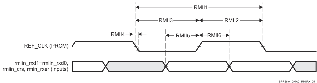
图 6-14. GMAC Receive Interface Timing RMII In operation
