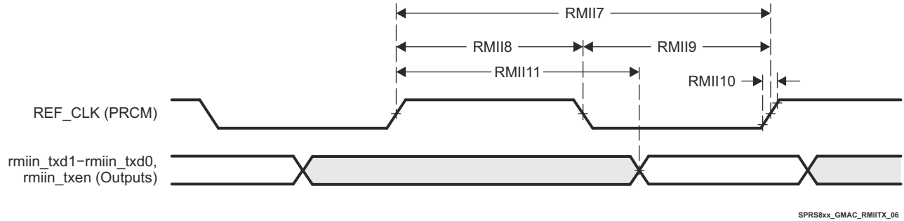
图 6-13. GMAC Transmit Interface Timing RMII In Operation
