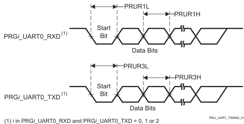
图 7-63. PRU-ICSS UART Timing Requirements and Switching Characteristics
