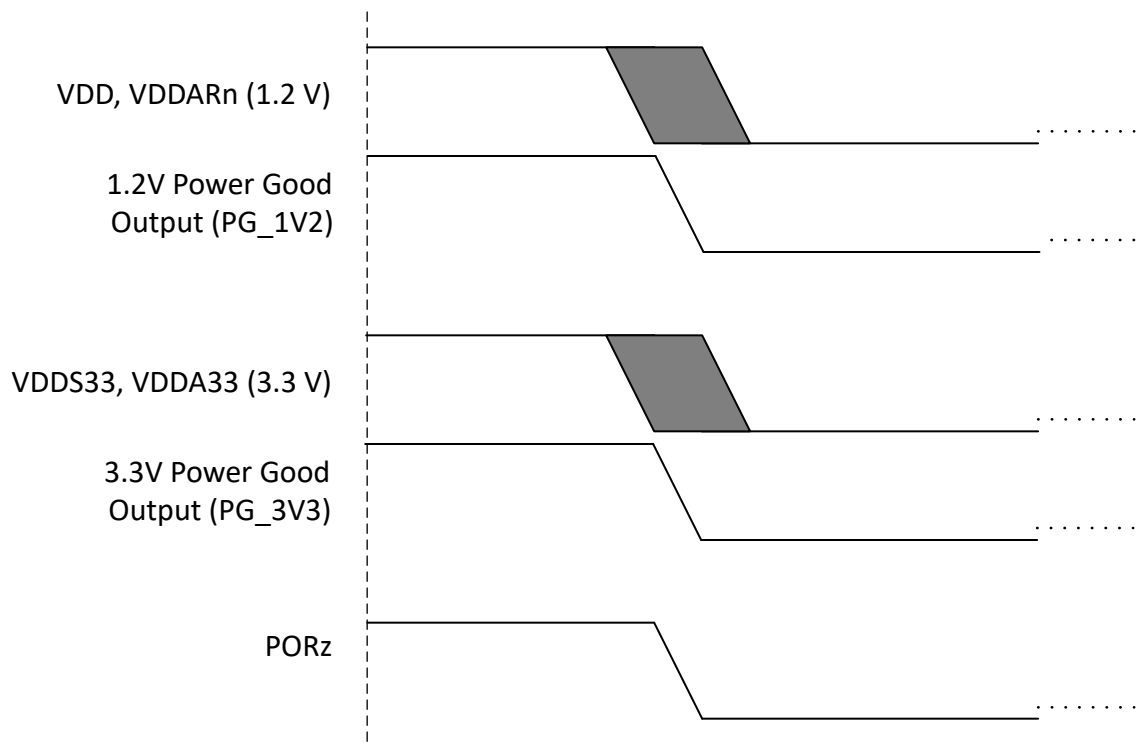
图 7-2. Power-Down Sequencing
