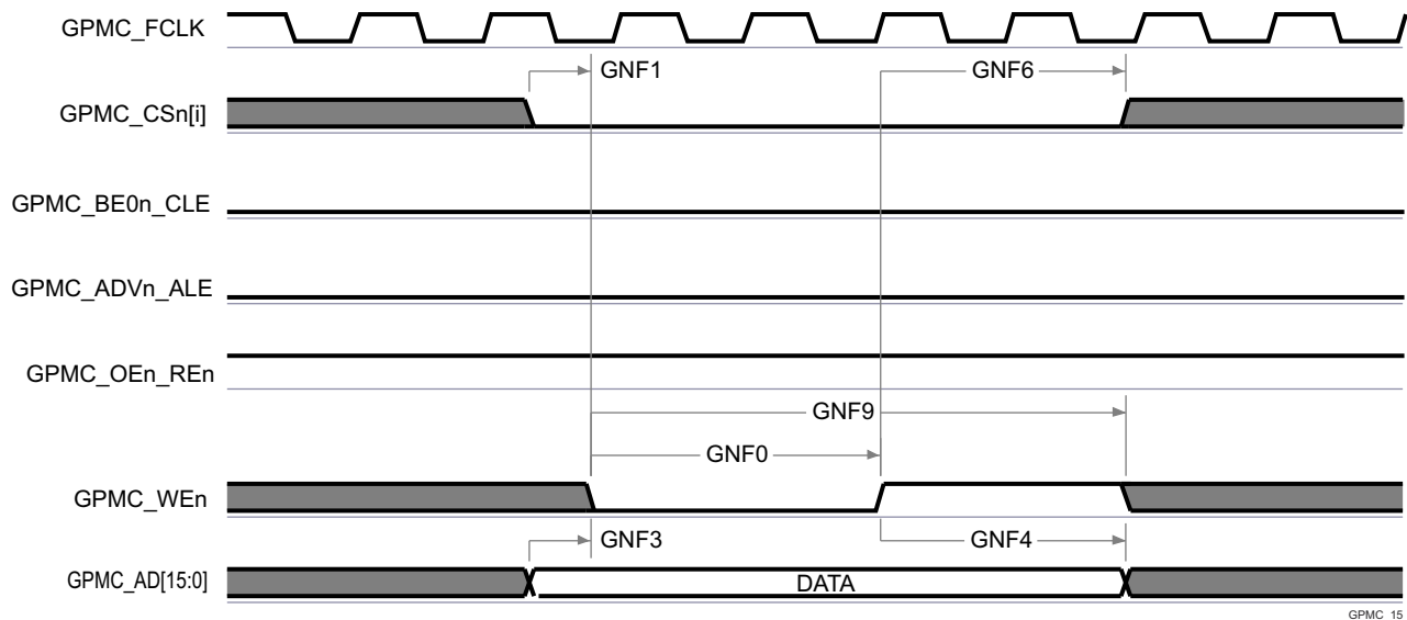
图 7-38. GPMC and NAND Flash — Data Read Cycle
