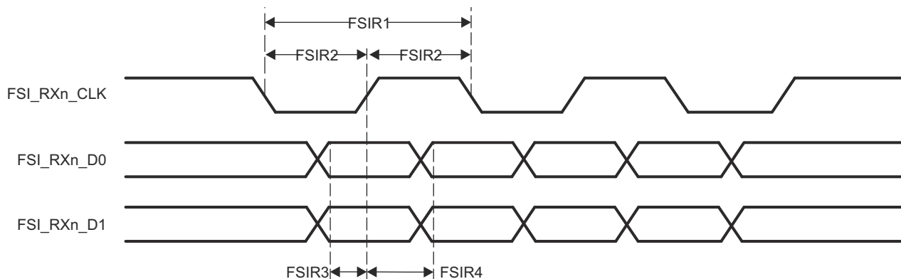
图 7-22. FSI Timing Requirements
