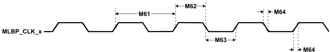
图 5-55. MLB_CLKP/N Timing (1)
