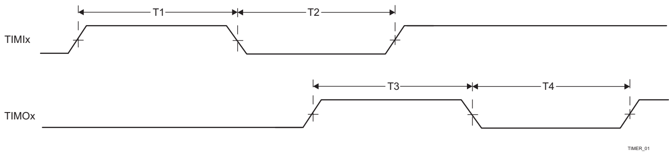
图 5-88. Timer Timing
