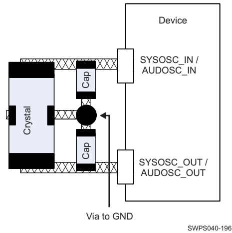
图 7-25. SYSOSC and AUDIOOSC PCB requirements
