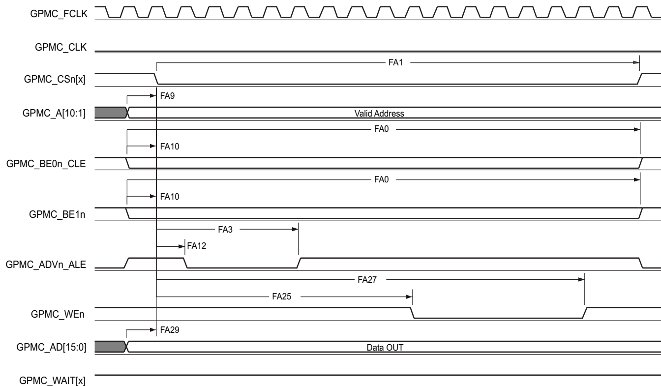
图 5-44. GPMC and NOR Flash—Asynchronous Write—Single Word
