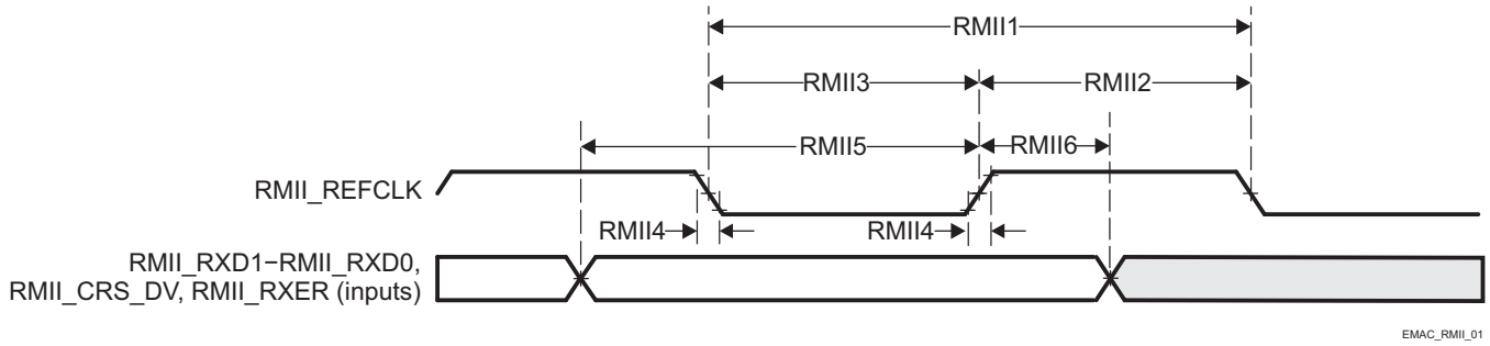
图 5-30. EMAC Receive Interface Timing RMII operation
