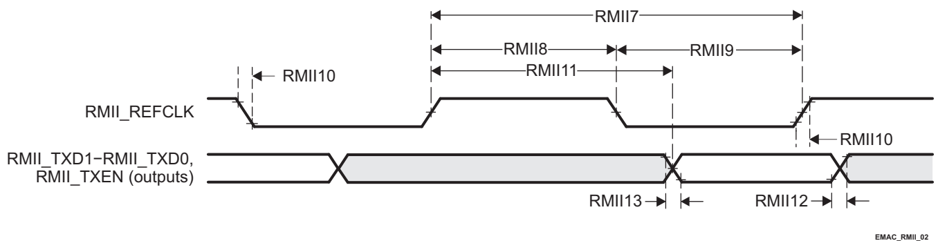
图 5-31. EMAC Transmit Interface Timing RMII Operation
