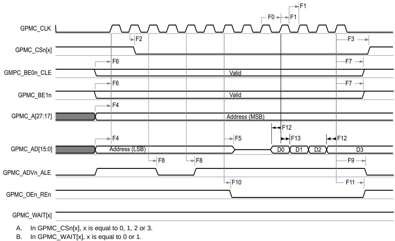
图 5-39. GPMC and Multiplexed NOR Flash—Synchronous Burst Read
