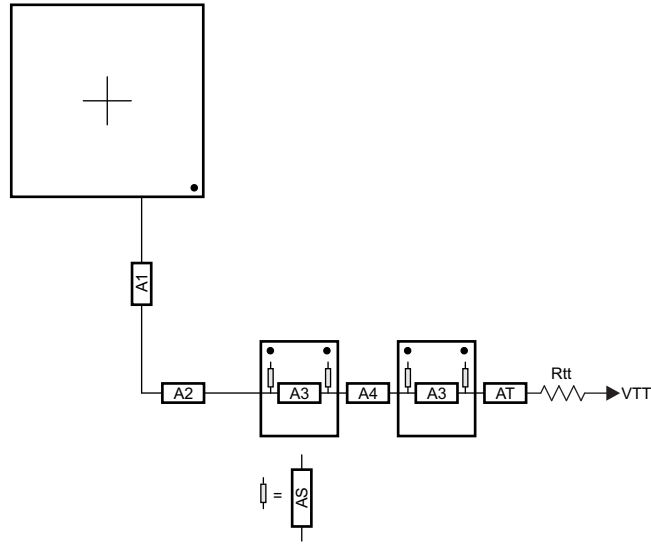
图 7-11. ADDR_CTRL Routing for Four Mirrored DDR3L Devices
